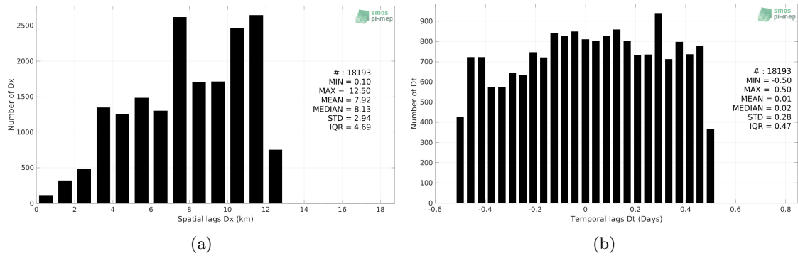
Figure 5: Histograms of the spatial (a) and temporal (b) lags between the location/time of the TSG (SAMOS) measurement and the date of the corresponding SMOS SSS L3 v332 - 9 Days (CATDS-CPDC) SSS pixel.
