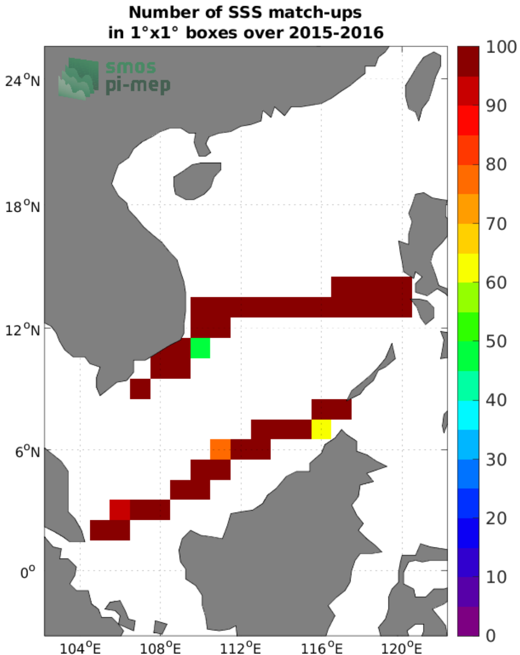
Figure 4: Number of SSS match-ups between TSG (SAMOS) SSS and the SMOS SSS L3 v332 - 9 Days (CATDS-CPDC) SSS product for the South China Sea Pi-MEP region over 1°x1° boxes and for the full satellite product period.
