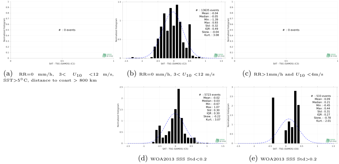
Figure 13: Normalized histogram of \Delta SSS (SMOS SSS L3 v332 - 9 Days (CATDS-CPDC) - TSG (SAMOS)) for 5 different subdatasets corresponding to: RR=0 mm/h, 3 < U_{10} < 12 m/s, SST > 5°C, distance to coast > 800 km (a), RR=0 mm/h, 3 < U_{10} < 12 m/s (b), RR > 1mm/h and U_{10} < 4 m/s (c), WOA2013 SSS Std < 0.2 (d), WOA2013 SSS Std > 0.2 (e).
