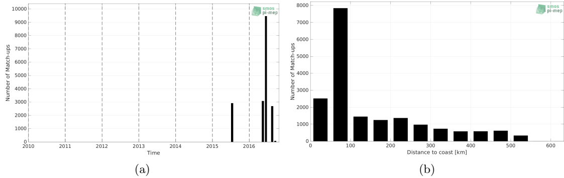
Figure 1: Number of match-ups between TSG (SAMOS) and SMOS SSS L3 v332 - 9 Days (CATDS-CPDC) SSS as a function of time (a) and as function of the distance to coast (b) over the South China Sea Pi-MEP region and for the full satellite product period.
