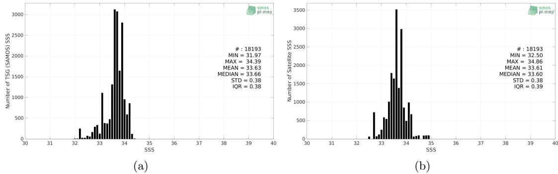
Figure 2: Histograms of SSS from TSG (SAMOS) (a) and SMOS SSS L3 v332 - 9 Days (CATDS-CPDC) (b) considering all match-up pairs per bins of 0.1 over the South China Sea Pi-MEP region and for the full satellite product period.
