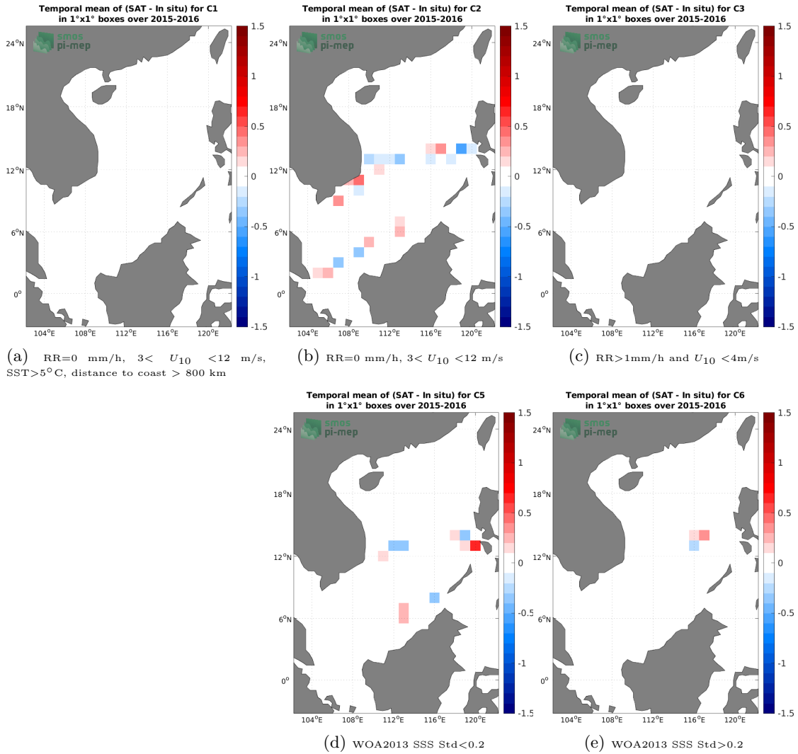
Figure 12: Temporal mean gridded over spatial boxes of size 1^\circ \times 1^\circ of \Delta SSS (SMOS SSS L3 v332 - 9 Days (CATDS-CPDC) - TSG (SAMOS)) for 5 different subdatasets corresponding to:RR=0 mm/h, 3 < U_{10} < 12 m/s, SST>5°C, distance to coast > 800 km (a), RR=0 mm/h, 3 < U_{10} < 12 m/s (b), RR>1mm/h and U_{10} < 4 m/s (c), WOA2013 SSS Std<0.2 (d), WOA2013 SSS Std>0.2 (e).
