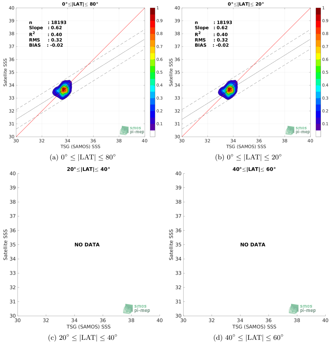
Figure 9: Contour maps of the concentration of SMOS SSS L3 v332 - 9 Days (CATDS-CPDC) SSS (y-axis) versus TSG (SAMOS) SSS (x-axis) at match-up pairs for different latitude bands. For each plot, the red line shows x=y . The black thin and dashed lines indicate a linear fit through the data cloud and the \pm 95\% confidence levels, respectively. The number match-up pairs n , the slope and R^2 coefficient of the linear fit, the root mean square (RMS) and the mean bias between satellite and in situ data are indicated for each latitude band in each plots.
