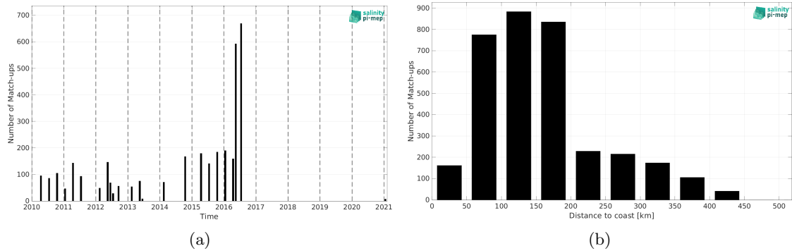
Figure 2: Number of match-ups between TSG (LEGOS-DM) and SMOS SSS L3 v332 - 9 Days (CATDS-CPDC) SSS as a function of time (a) and as function of the distance to coast (b) over the South China Sea Pi-MEP region and for the full satellite product period.
