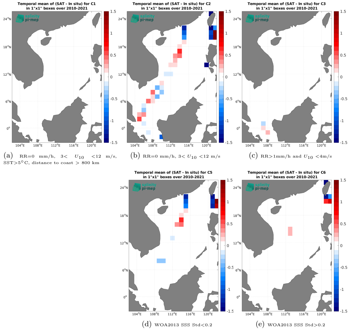
Figure 14: Temporal mean gridded over spatial boxes of size 1^\circ \times 1^\circ of \Delta SSS (SMOS SSS L3 v332 - 9 Days (CATDS-CPDC) - TSG (LEGOS-DM)) for 5 different subdatasets corresponding to: RR=0 mm/h, 3 < U_{10} < 12 m/s, SST>5°C, distance to coast > 800 km (a), RR=0 mm/h, 3 < U_{10} < 12 m/s (b), RR>1mm/h and U_{10} < 4 m/s (c), WOA2013 SSS Std<0.2 (d), WOA2013 SSS Std>0.2 (e).
