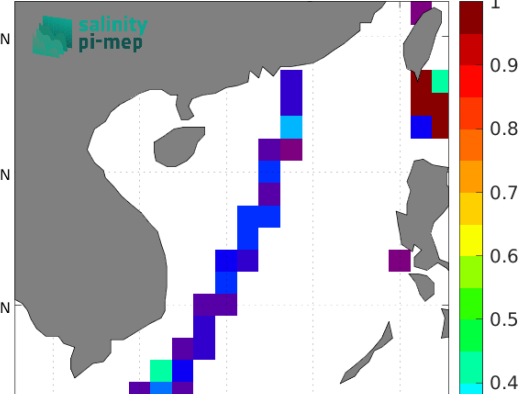
Temporal STD of (Sat - TSG (LEGOS-DM)) in 1°x1° boxes over 2010-2021
