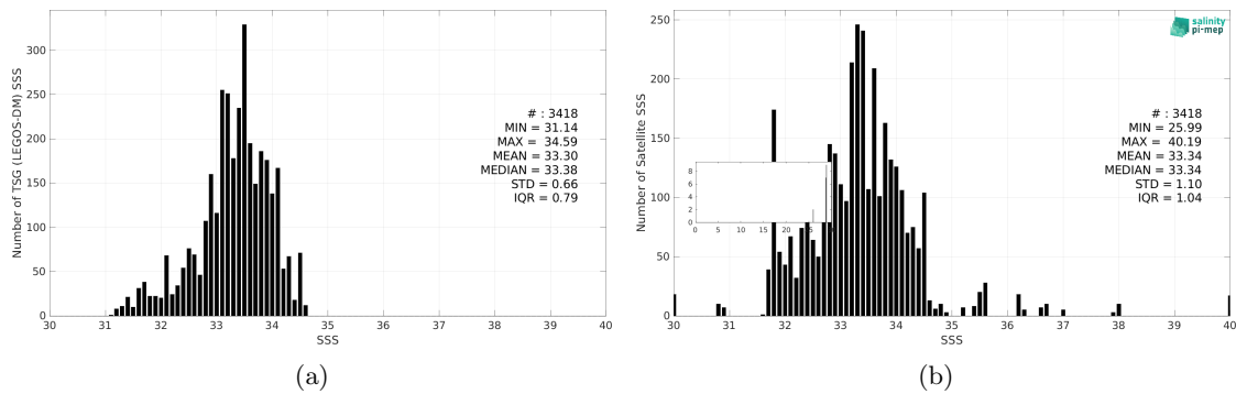
Figure 3: Histograms of SSS from TSG (LEGOS-DM) (a) and SMOS SSS L3 v332 - 9 Days (CATDS-CPDC) (b) considering all match-up pairs per bins of 0.1 over the South China Sea Pi-MEP region and for the full satellite product period.
