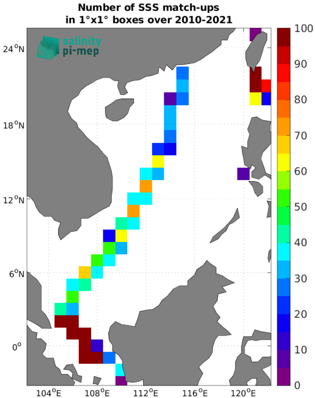
Figure 5: Number of SSS match-ups between TSG (LEGOS-DM) SSS and the SMOS SSS L3 v332 - 9 Days (CATDS-CPDC) SSS product for the South China Sea Pi-MEP region over 1^{\circ} \times 1^{\circ} boxes and for the full satellite product period.
