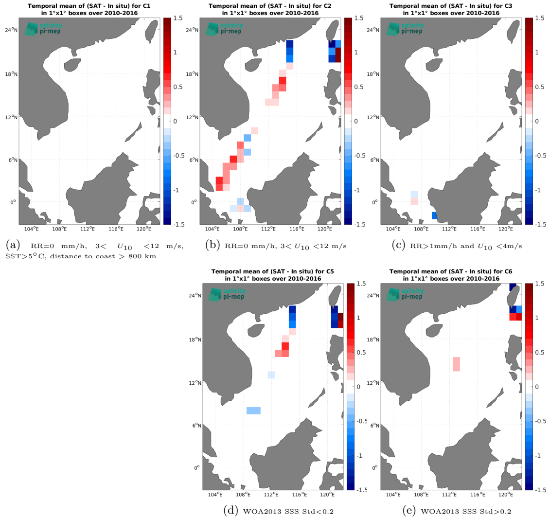
Figure 12: Temporal mean gridded over spatial boxes of size 1^\circ \times 1^\circ of \Delta\text{SSS} (SMOS SSS L3 v332 - 9 Days (CATDS-CPDC) - TSG (LEGOS-DM)) for 5 different subdatasets corresponding to: RR=0 mm/h, 3 < U_{10} < 12 m/s, SST > 5^\circ\text{C} , distance to coast > 800 km (a), RR=0 mm/h, 3 < U_{10} < 12 m/s (b), RR > 1 mm/h and U_{10} < 4 m/s (c), WOA2013 SSS Std < 0.2 (d), WOA2013 SSS Std > 0.2 (e).
