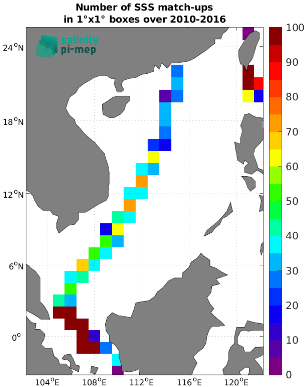
Figure 4: Number of SSS match-ups between TSG (LEGOS-DM) SSS and the SMOS SSS L3 v332 - 9 Days (CATDS-CPDC) SSS product for the South China Sea Pi-MEP region over 1^{\circ} \times 1^{\circ} boxes and for the full satellite product period.
