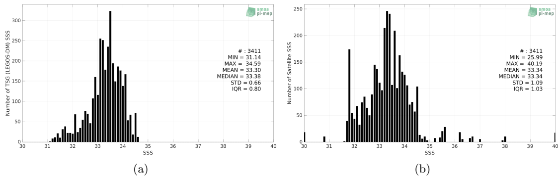
Figure 2: Histograms of SSS from TSG (LEGOS-DM) (a) and SMOS SSS L3 v332 - 9 Days (CATDS-CPDC) (b) considering all match-up pairs per bins of 0.1 over the South China Sea Pi-MEP region and for the full satellite product period.
