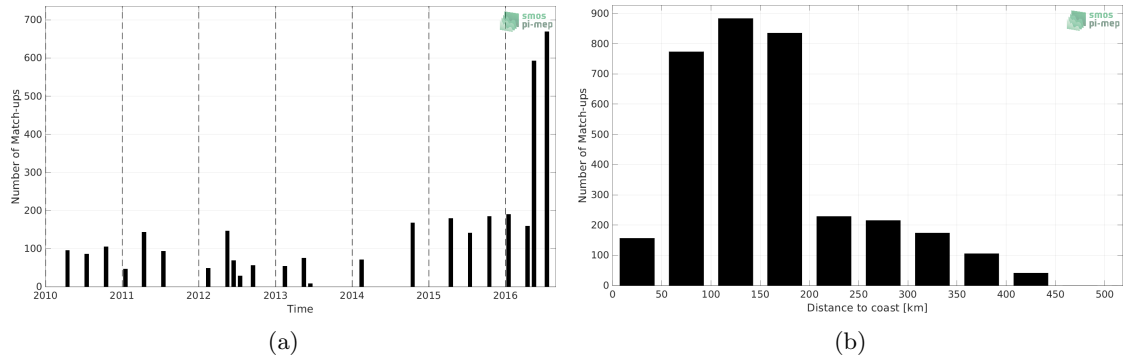
Figure 1: Number of match-ups between TSG (LEGOS-DM) and SMOS SSS L3 v332 - 9 Days (CATDS-CPDC) SSS as a function of time (a) and as function of the distance to coast (b) over the South China Sea Pi-MEP region and for the full satellite product period.
