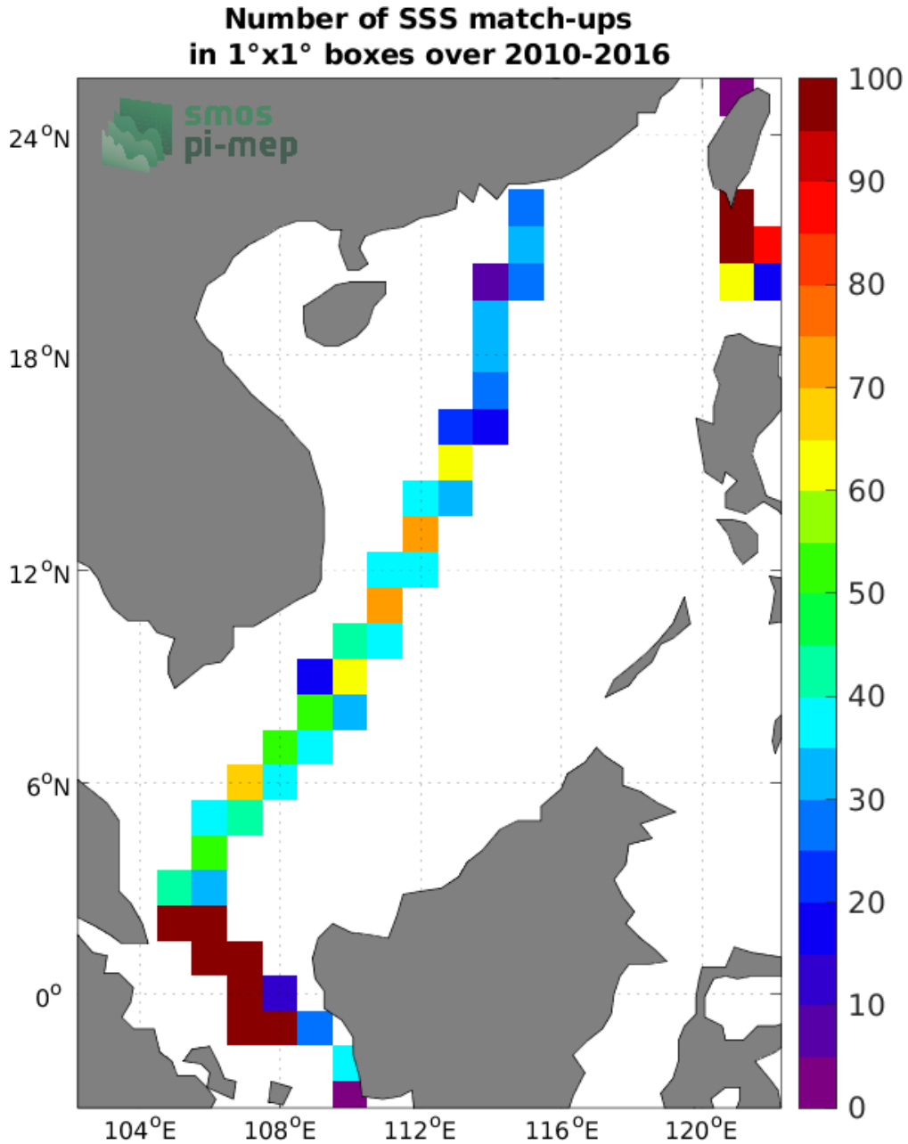
Figure 4: Number of SSS match-ups between TSG (LEGOS-DM) SSS and the SMOS SSS L3 v332 - 9 Days (CATDS-CPDC) SSS product for the South China Sea Pi-MEP region over 1^\circ \times 1^\circ boxes and for the full satellite product period.
