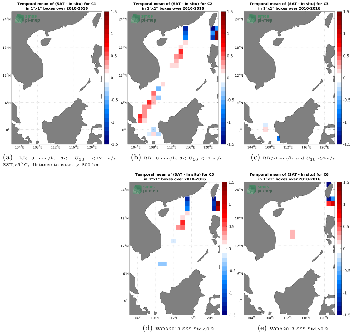
Figure 12: Temporal mean gridded over spatial boxes of size 1^\circ \times 1^\circ of \Delta SSS (SMOS SSS L3 v332 - 9 Days (CATDS-CPDC) - TSG (LEGOS-DM)) for 5 different subdatasets corresponding to:RR=0 mm/h, 3 < U_{10} < 12 m/s, SST>5°C, distance to coast > 800 km (a), RR=0 mm/h, 3 < U_{10} < 12 m/s (b), RR>1mm/h and U_{10} < 4 m/s (c), WOA2013 SSS Std<0.2 (d), WOA2013 SSS Std>0.2 (e).
