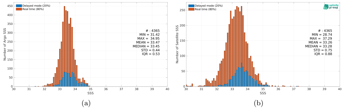
Figure 2: Histograms of SSS from Argo (a) and SMOS SSS L3 v332 - 9 Days (CATDS-CPDC) (b) considering all match-up pairs per bins of 0.1 over the South China Sea Pi-MEP region and for the full satellite product period.
