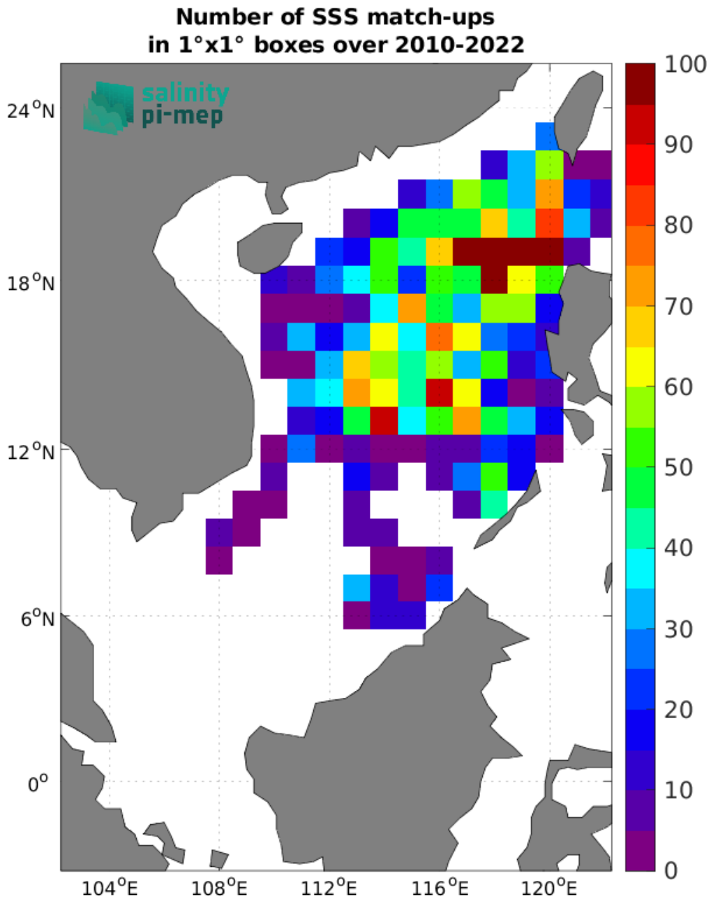
Figure 4: Number of SSS match-ups between Argo SSS and the SMOS SSS L3 v332 - 9 Days (CATDS-CPDC) SSS product for the South China Sea Pi-MEP region over 1^\circ \times 1^\circ boxes and for the full satellite product period.
