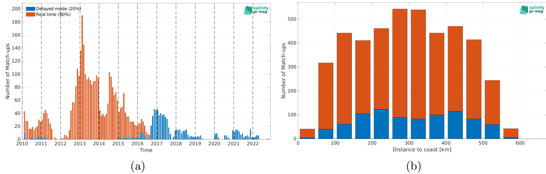
Figure 1: Number of match-ups between Argo and SMOS SSS L3 v332 - 9 Days (CATDS-CPDC) SSS as a function of time (a) and as function of the distance to coast (b) over the South China Sea Pi-MEP region and for the full satellite product period.
