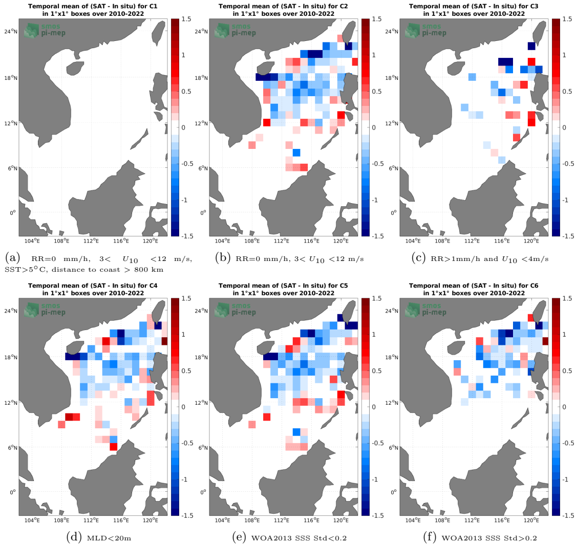
Figure 12: Temporal mean gridded over spatial boxes of size 1^\circ \times 1^\circ of \Delta\text{SSS} (SMOS SSS L3 v332 - 9 Days (CATDS-CPDC) - Argo) for 6 different subdatasets corresponding to: RR=0 mm/h, 3 < U_{10} < 12 m/s, SST > 5^\circ\text{C} , distance to coast > 800 km (a), RR=0 mm/h, 3 < U_{10} < 12 m/s (b), RR > 1 mm/h and U_{10} < 4 m/s (c), MLD < 20 m (d), WOA2013 SSS Std < 0.2 (e), WOA2013 SSS Std > 0.2 (f).
