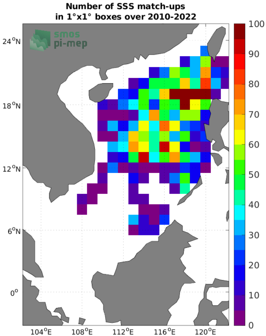
Figure 4: Number of SSS match-ups between Argo SSS and the SMOS SSS L3 v332 - 9 Days (CATDS-CPDC) SSS product for the South China Sea Pi-MEP region over 1°x1° boxes and for the full satellite product period.
