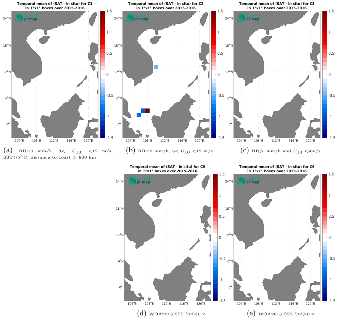
Figure 12: Temporal mean gridded over spatial boxes of size 1^\circ \times 1^\circ of \Delta\text{SSS} (SMOS SSS L2Q v331 - 0.25 Deg (CATDS-CPDC) - TSG (SAMOS)) for 5 different subdatasets corresponding to: RR=0 mm/h, 3 < U_{10} < 12 m/s, SST > 5^\circ\text{C} , distance to coast > 800 km (a), RR=0 mm/h, 3 < U_{10} < 12 m/s (b), RR > 1 mm/h and U_{10} < 4 m/s (c), WOA2013 SSS Std < 0.2 (d), WOA2013 SSS Std > 0.2 (e).
