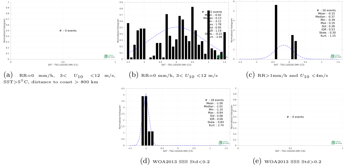
Figure 13: Normalized histogram of \Delta\text{SSS} (SMOS SSS L2Q v331 - 0.25 Deg (CATDS-CPDC) - TSG (LEGOS-DM)) for 5 different subdatasets corresponding to: RR=0 mm/h, 3 < U_{10} < 12 m/s, SST > 5^{\circ}\text{C} , distance to coast > 800 km (a), RR=0 mm/h, 3 < U_{10} < 12 m/s (b), RR > 1\text{mm/h} and U_{10} < 4\text{m/s} (c), WOA2013 SSS Std < 0.2 (d), WOA2013 SSS Std > 0.2 (e).
