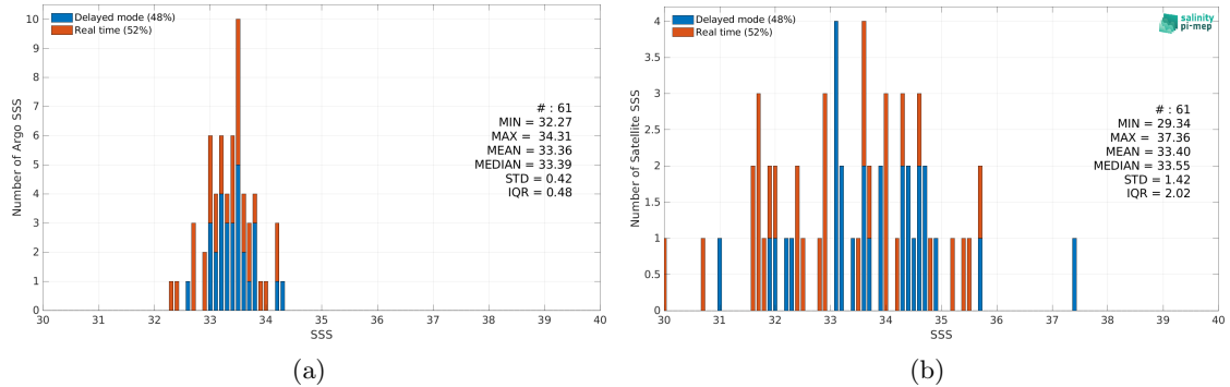
Figure 2: Histograms of SSS from Argo (a) and SMOS SSS L2Q v331 - 0.25 Deg (CATDS-CPDC) (b) considering all match-up pairs per bins of 0.1 over the South China Sea Pi-MEP region and for the full satellite product period.
