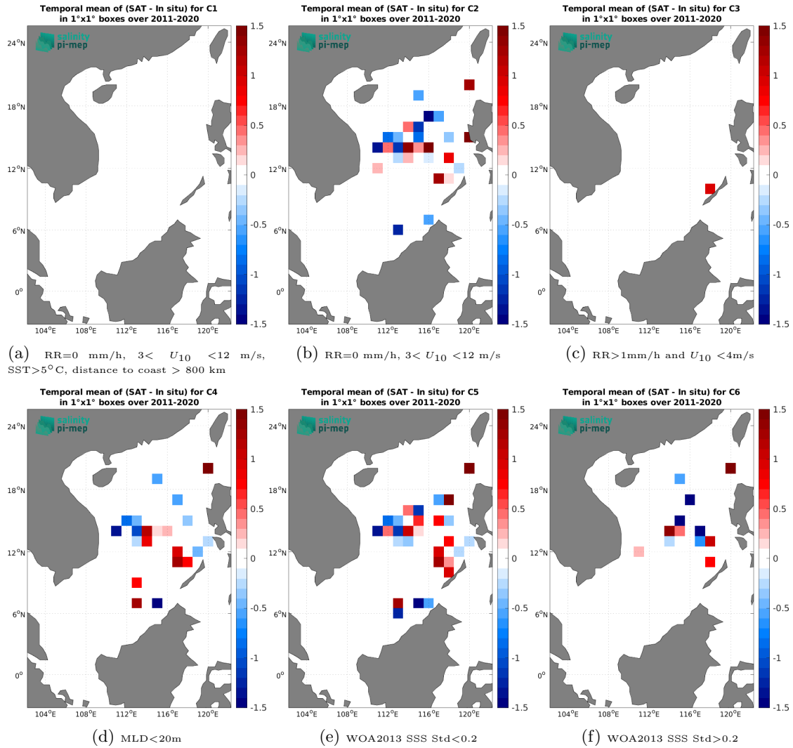
Figure 12: Temporal mean gridded over spatial boxes of size 1^\circ \times 1^\circ of \Delta SSS (SMOS SSS L2Q v331 - 0.25 Deg (CATDS-CPDC) - Argo) for 6 different subdatasets corresponding to: RR=0 mm/h, 3 < U_{10} < 12 m/s, SST > 5^\circ\text{C} , distance to coast > 800 km (a), RR=0 mm/h, 3 < U_{10} < 12 m/s (b), RR > 1 mm/h and U_{10} < 4 m/s (c), MLD < 20 m (d), WOA2013 SSS Std < 0.2 (e), WOA2013 SSS Std > 0.2 (f).
