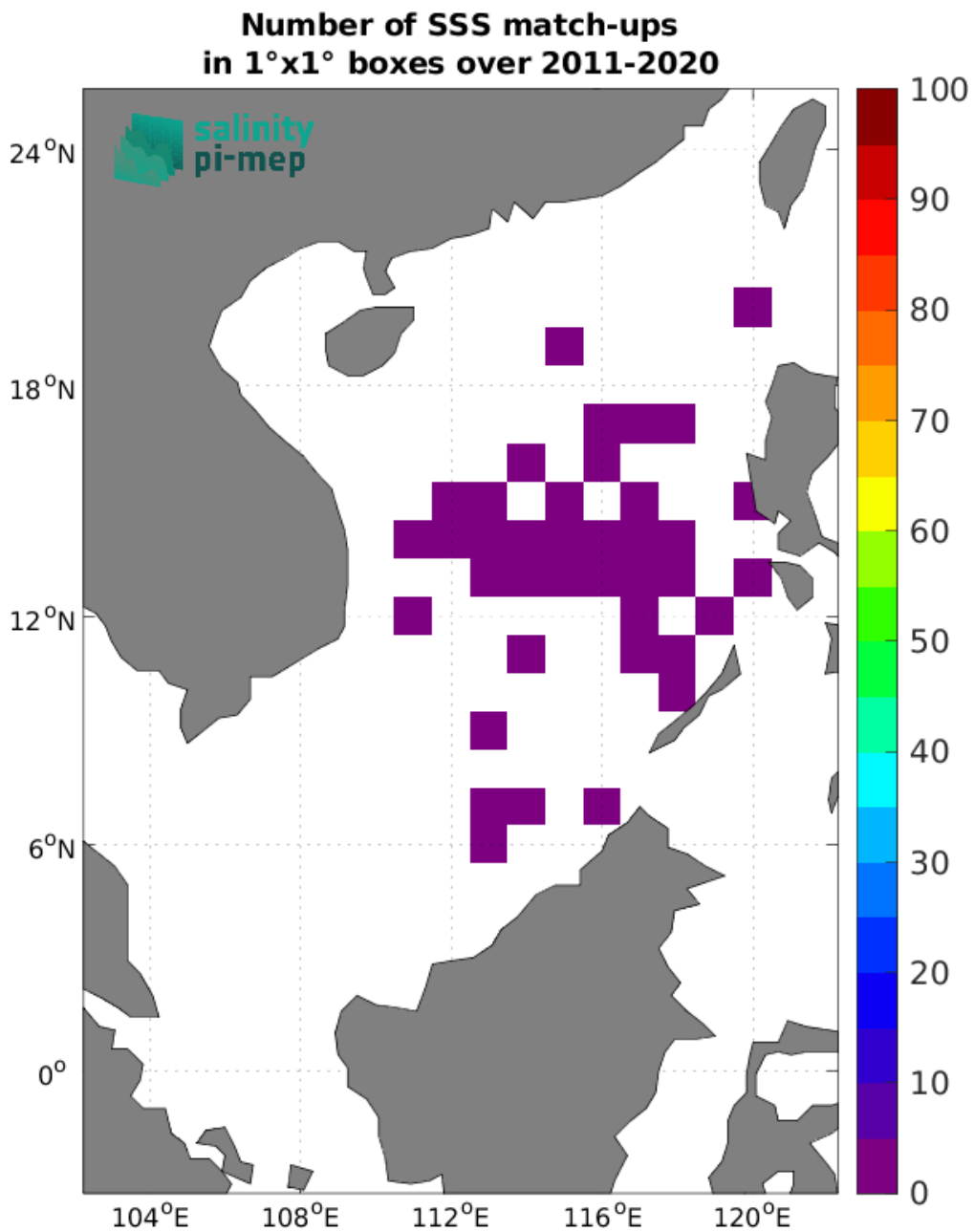
Figure 4: Number of SSS match-ups between Argo SSS and the SMOS SSS L2Q v331 - 0.25 Deg (CATDS-CPDC) SSS product for the South China Sea Pi-MEP region over 1^{\circ} \times 1^{\circ} boxes and for the full satellite product period.
