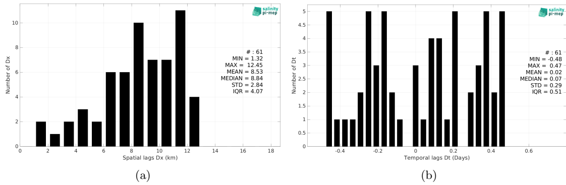
Figure 5: Histograms of the spatial (a) and temporal (b) lags between the location/time of the Argo measurement and the date of the corresponding SMOS SSS L2Q v331 - 0.25 Deg (CATDS-CPDC) SSS pixel.
