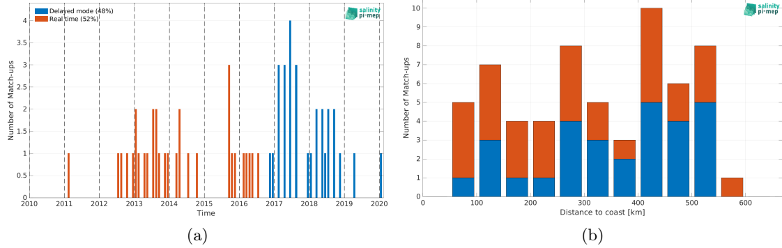
Figure 1: Number of match-ups between Argo and SMOS SSS L2Q v331 - 0.25 Deg (CATDS-CPDC) SSS as a function of time (a) and as function of the distance to coast (b) over the South China Sea Pi-MEP region and for the full satellite product period.
