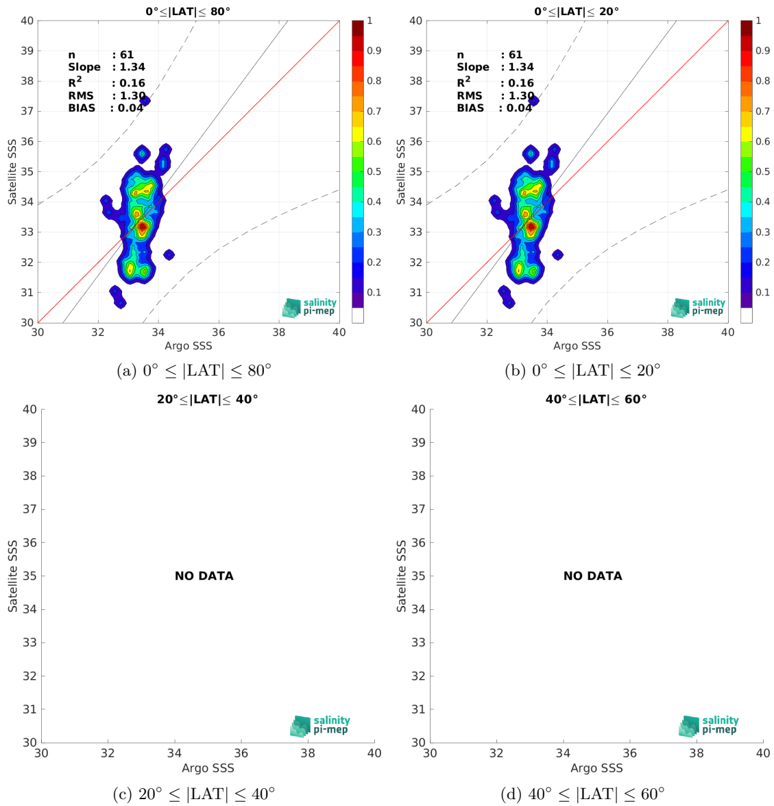
Figure 9: Contour maps of the concentration of SMOS SSS L2Q v331 - 0.25 Deg (CATDS-CPDC) SSS (y-axis) versus Argo SSS (x-axis) at match-up pairs for different latitude bands. For each plot, the red line shows x=y . The black thin and dashed lines indicate a linear fit through the data cloud and the \pm 95\% confidence levels, respectively. The number match-up pairs n , the slope and R^2 coefficient of the linear fit, the root mean square (RMS) and the mean bias between satellite and in situ data are indicated for each latitude band in each plots.
