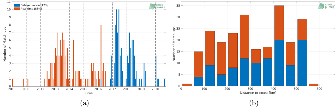
Figure 1: Number of match-ups between Argo and SMOS SSS L2Q v331 - 0.25 Deg (CATDS-CPDC) SSS as a function of time (a) and as function of the distance to coast (b) over the South China Sea Pi-MEP region and for the full satellite product period.
