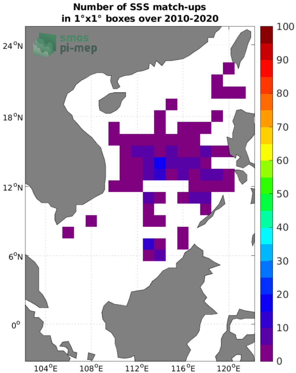
Figure 4: Number of SSS match-ups between Argo SSS and the SMOS SSS L2Q v331 - 0.25 Deg (CATDS-CPDC) SSS product for the South China Sea Pi-MEP region over 1°x1° boxes and for the full satellite product period.
