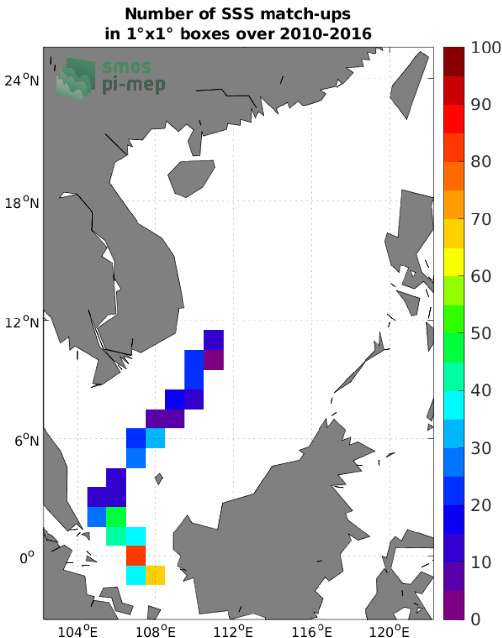
Figure 4: Number of SSS match-ups between TSG (LEGOS-DM) SSS and the SMOS SSS L2Q v330 - 0.25 Deg (CATDS-CPDC) SSS product for the South China Sea Pi-MEP region over 1°x1° boxes and for the full satellite product period.
