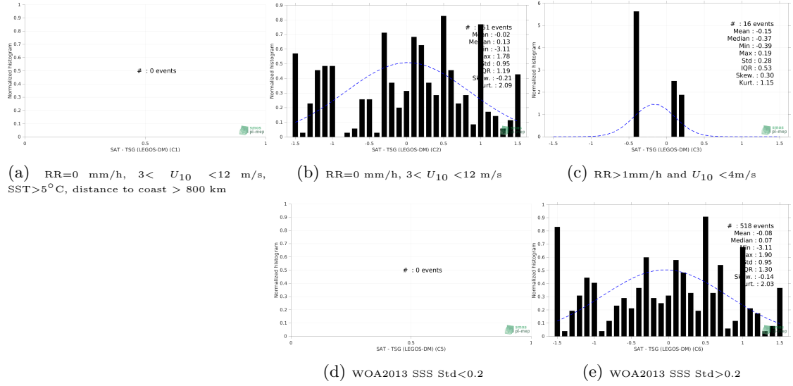
Figure 13: Normalized histogram of \Delta\text{SSS} (SMOS SSS L2Q v330 - 0.25 Deg (CATDS-CPDC) - TSG (LEGOS-DM)) for 5 different subdatasets corresponding to: RR=0 mm/h, 3 < U_{10} < 12 m/s, SST > 5^{\circ}\text{C} , distance to coast > 800 km (a), RR=0 mm/h, 3 < U_{10} < 12 m/s (b), RR > 1\text{mm/h} and U_{10} < 4\text{m/s} (c), WOA2013 SSS Std < 0.2 (d), WOA2013 SSS Std > 0.2 (e).
