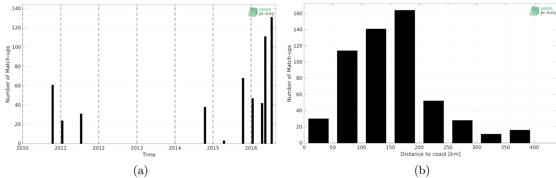
Figure 1: Number of match-ups between TSG (LEGOS-DM) and SMOS SSS L2Q v330 - 0.25 Deg (CATDS-CPDC) SSS as a function of time (a) and as function of the distance to coast (b) over the South China Sea Pi-MEP region and for the full satellite product period.
