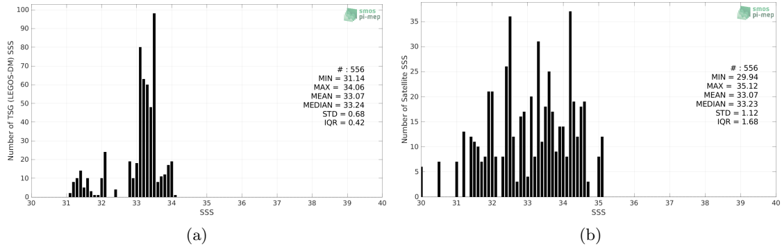
Figure 2: Histograms of SSS from TSG (LEGOS-DM) (a) and SMOS SSS L2Q v330 - 0.25 Deg (CATDS-CPDC) (b) considering all match-up pairs per bins of 0.1 over the South China Sea Pi-MEP region and for the full satellite product period.
