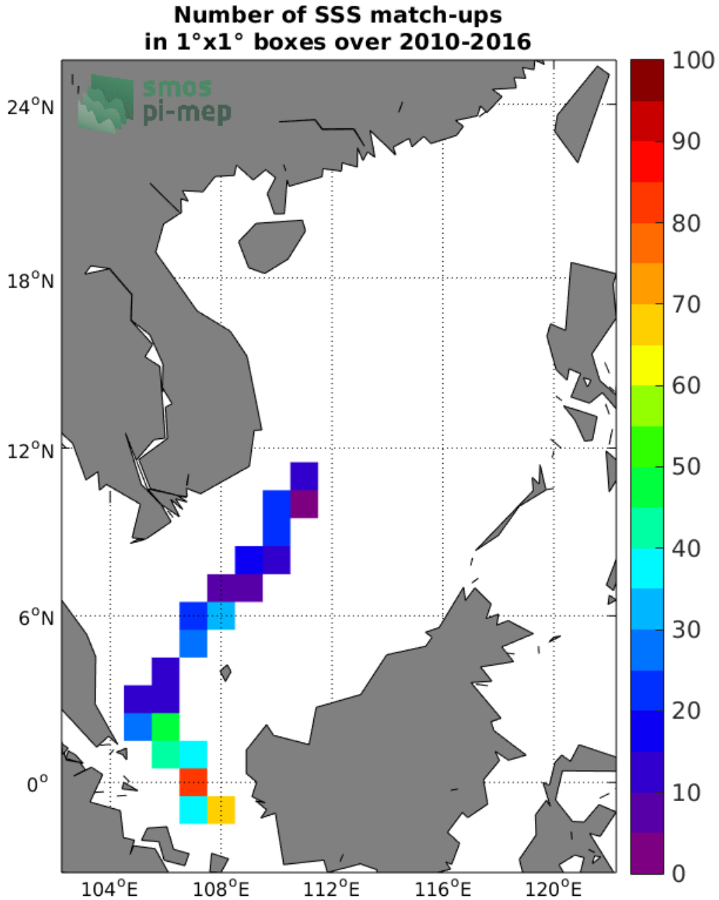
Figure 4: Number of SSS match-ups between TSG (LEGOS-DM) SSS and the SMOS SSS L2Q v330 - 0.25 Deg (CATDS-CPDC) SSS product for the South China Sea Pi-MEP region over 1^\circ \times 1^\circ boxes and for the full satellite product period.
