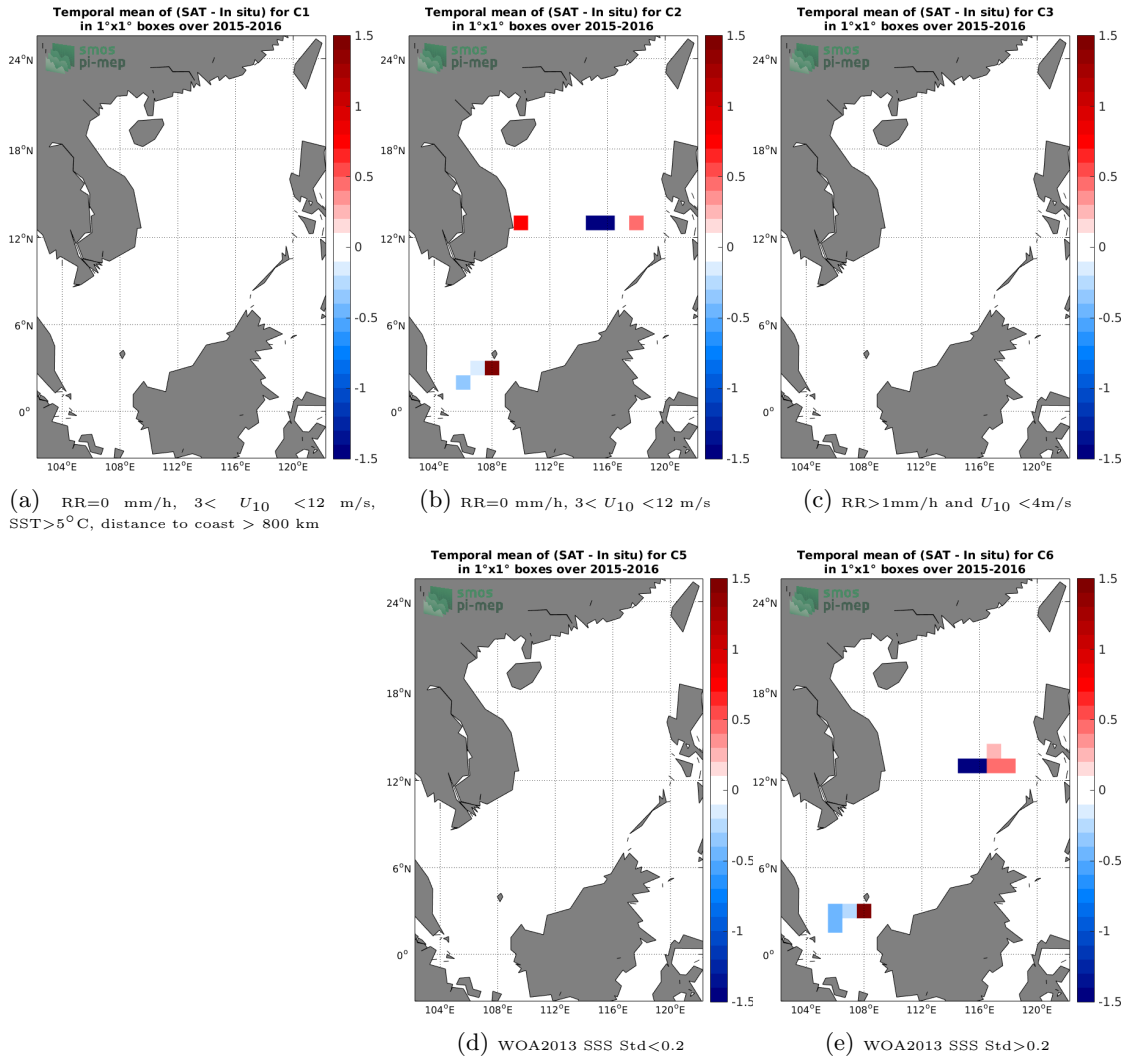
Figure 12: Temporal mean gridded over spatial boxes of size 1^\circ \times 1^\circ of \Delta SSS (SMOS SSS L2Q v321 - 0.25 Deg (CATDS-CPDC) - TSG (SAMOS)) for 5 different subdatasets corresponding to: RR=0 mm/h, 3 < U_{10} < 12 m/s, SST>5°C, distance to coast > 800 km (a), RR=0 mm/h, 3 < U_{10} < 12 m/s (b), RR>1mm/h and U_{10} < 4 m/s (c), WOA2013 SSS Std<0.2 (d), WOA2013 SSS Std>0.2 (e).
