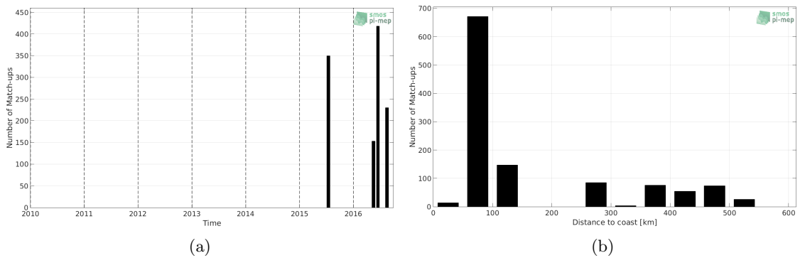
Figure 1: Number of match-ups between TSG (SAMOS) and SMOS SSS L2Q v321 - 0.25 Deg (CATDS-CPDC) SSS as a function of time (a) and as function of the distance to coast (b) over the South China Sea Pi-MEP region and for the full satellite product period.
