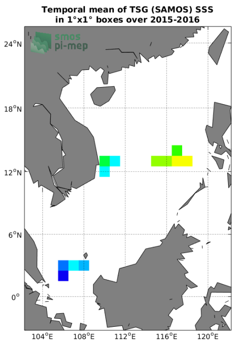
(c) MEAN(TSG (SAMOS) SSS)
