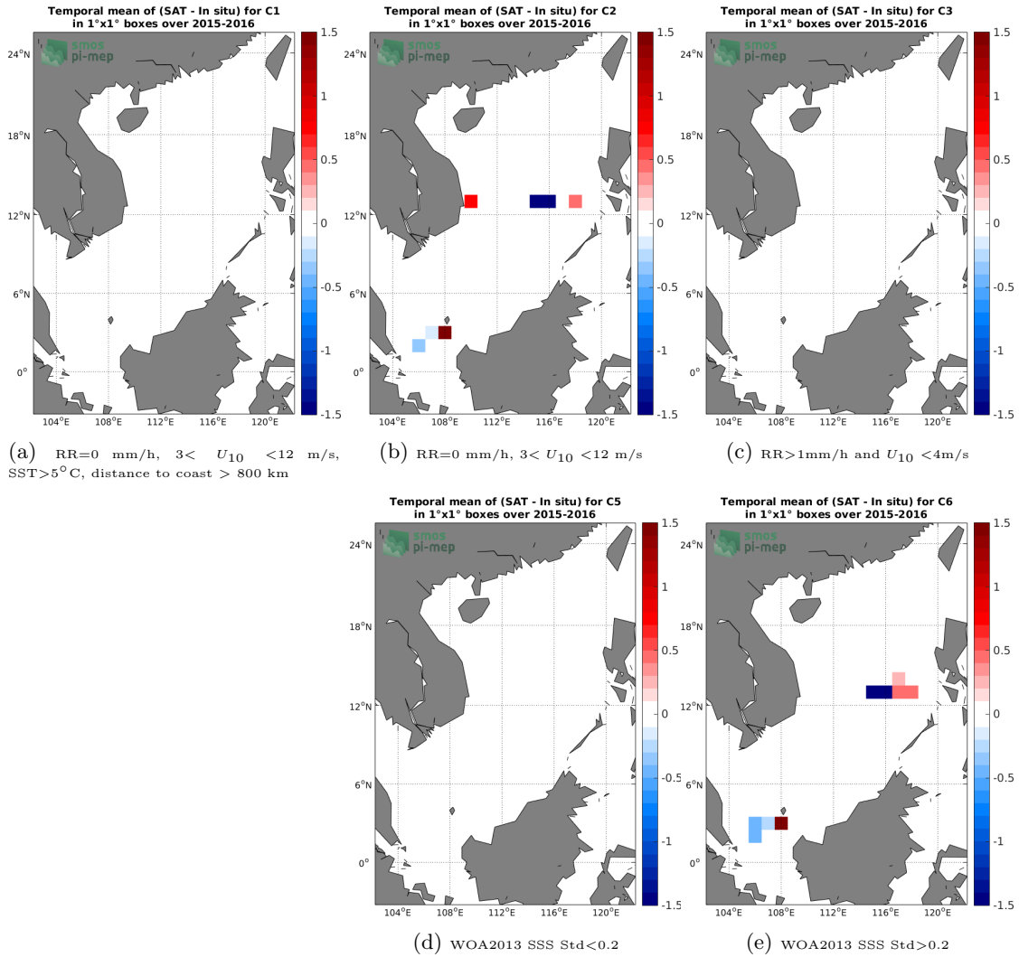
Figure 12: Temporal mean gridded over spatial boxes of size 1°x1° of \Delta SSS (SMOS SSS L2Q v321 - 0.25 Deg (CATDS-CPDC) - TSG (SAMOS)) for 5 different subdatasets corresponding to:RR=0 mm/h, 3 < U_{10} < 12 m/s, SST>5°C, distance to coast > 800 km (a), RR=0 mm/h, 3 < U_{10} < 12 m/s (b), RR>1mm/h and U_{10} < 4 m/s (c), WOA2013 SSS Std<0.2 (d), WOA2013 SSS Std>0.2 (e).
