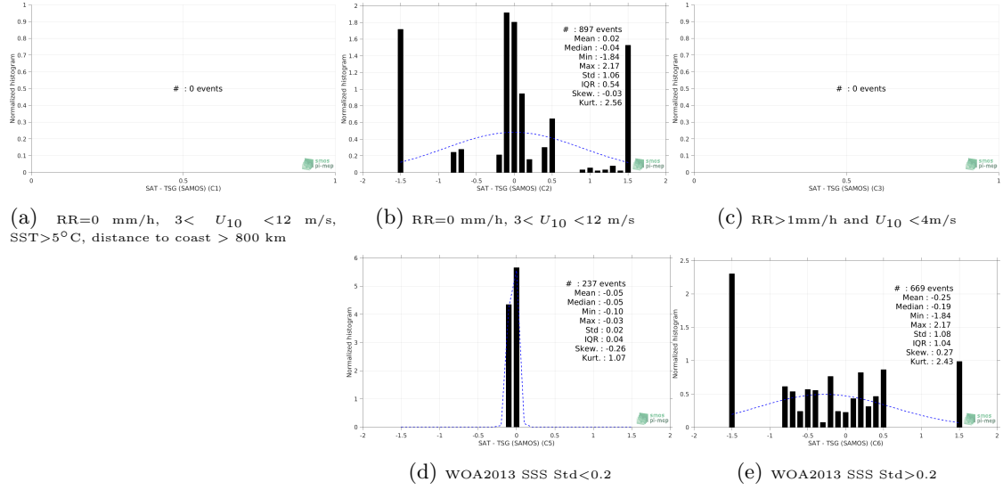
Figure 13: Normalized histogram of \Delta SSS (SMOS SSS L2Q v321 - 0.25 Deg (CATDS-CPDC) - TSG (SAMOS)) for 5 different subdatasets corresponding to: RR=0 mm/h, 3 < U_{10} < 12 m/s, SST > 5°C, distance to coast > 800 km (a), RR=0 mm/h, 3 < U_{10} < 12 m/s (b), RR > 1mm/h and U_{10} < 4 m/s (c), WOA2013 SSS Std < 0.2 (d), WOA2013 SSS Std > 0.2 (e).
