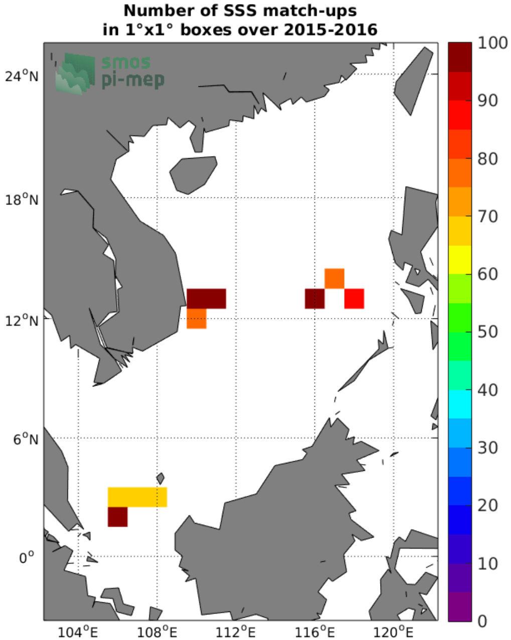
Figure 4: Number of SSS match-ups between TSG (SAMOS) SSS and the SMOS SSS L2Q v321 - 0.25 Deg (CATDS-CPDC) SSS product for the South China Sea Pi-MEP region over 1°x1° boxes and for the full satellite product period.
