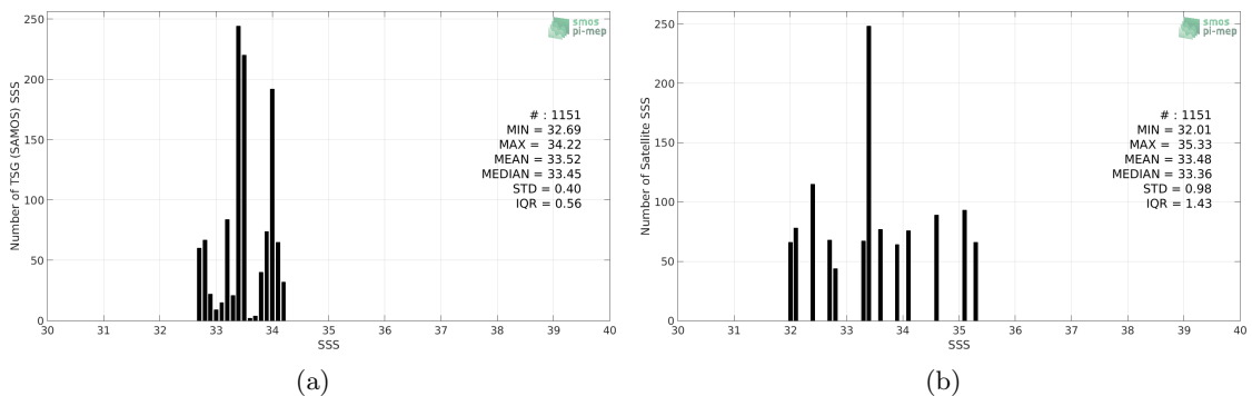
Figure 2: Histograms of SSS from TSG (SAMOS) (a) and SMOS SSS L2Q v321 - 0.25 Deg (CATDS-CPDC) (b) considering all match-up pairs per bins of 0.1 over the South China Sea Pi-MEP region and for the full satellite product period.
