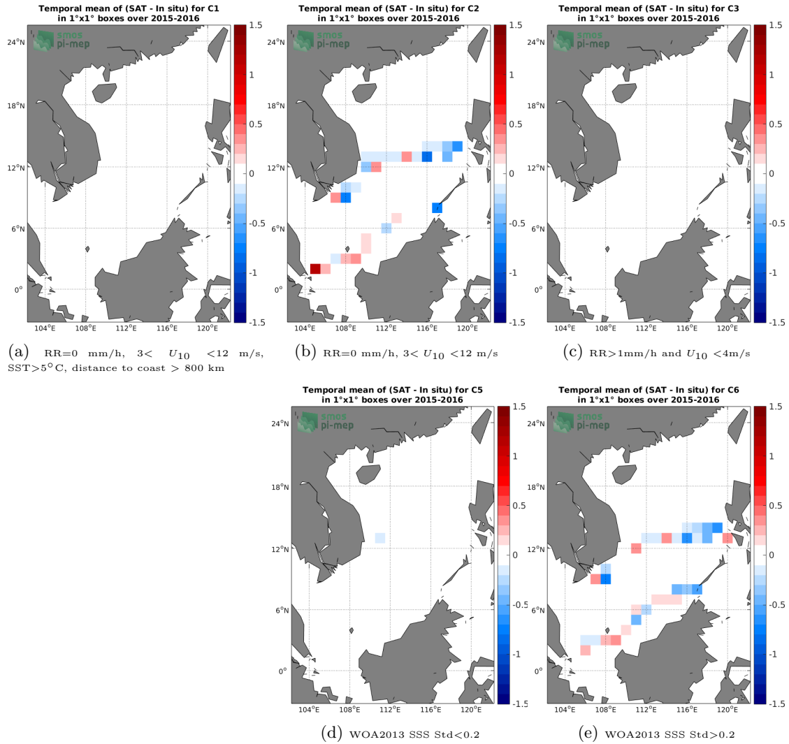
Figure 12: Temporal mean gridded over spatial boxes of size 1^\circ \times 1^\circ of \Delta SSS (SMOS SSS L3 v317 - Monthly - 25 km (CATDS-CPDC) - TSG (SAMOS)) for 5 different subdatasets corresponding to: RR=0 mm/h, 3 < U_{10} < 12 m/s, SST>5°C, distance to coast > 800 km (a), RR=0 mm/h, 3 < U_{10} < 12 m/s (b), RR>1mm/h and U_{10} < 4 m/s (c), WOA2013 SSS Std<0.2 (d), WOA2013 SSS Std>0.2 (e).
