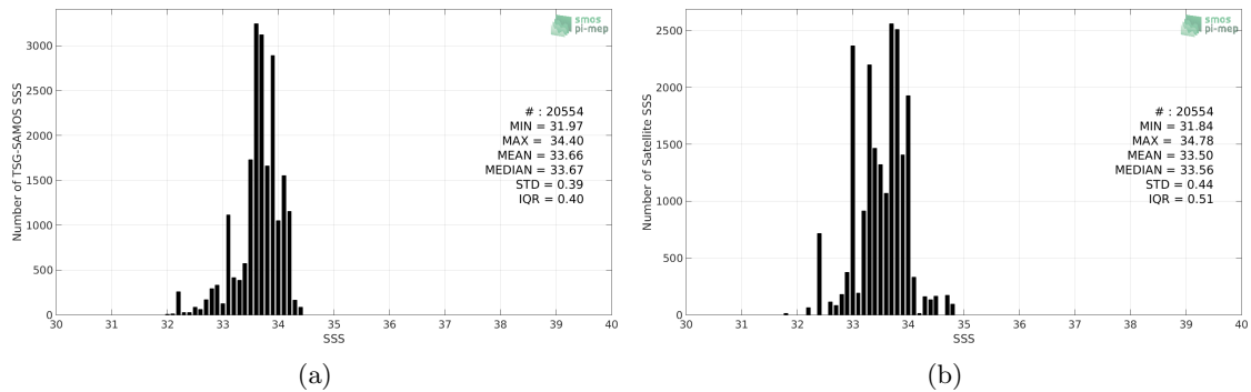
Figure 2: Histograms of SSS from TSG-SAMOS (a) and SMOS L3 v317 - Monthly - 25 km (CATDS-CPDC) (b) considering all match-up pairs per bins of 0.1 over the South China Sea Pi-MEP region and for the full satellite product period.
