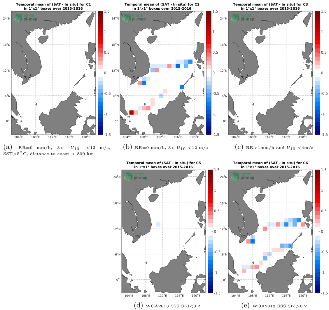
Figure 12: Temporal mean gridded over spatial boxes of size 1^\circ \times 1^\circ of \Delta SSS (SMOS L3 v317 - Monthly - 25 km (CATDS-CPDC) - TSG-SAMOS) for 5 different subdatasets corresponding to:RR=0 mm/h, 3 < U_{10} < 12 m/s, SST>5°C, distance to coast > 800 km (a), RR=0 mm/h, 3 < U_{10} < 12 m/s (b), RR>1mm/h and U_{10} < 4 m/s (c), WOA2013 SSS Std<0.2 (d), WOA2013 SSS Std>0.2 (e).
