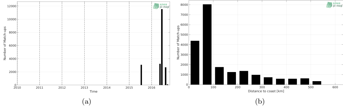
Figure 1: Number of match-ups between TSG-SAMOS and SMOS L3 v317 - Monthly - 25 km (CATDS-CPDC) SSS as a function of time (a) and as function of the distance to coast (b) over the South China Sea Pi-MEP region and for the full satellite product period.
