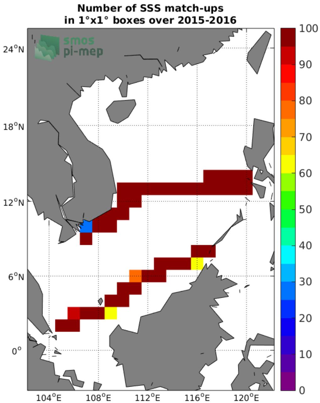
Figure 4: Number of SSS match-ups between TSG-SAMOS SSS and the SMOS L3 v317 - Monthly - 25 km (CATDS-CPDC) SSS product for the South China Sea Pi-MEP region over 1°x1° boxes and for the full satellite product period.
