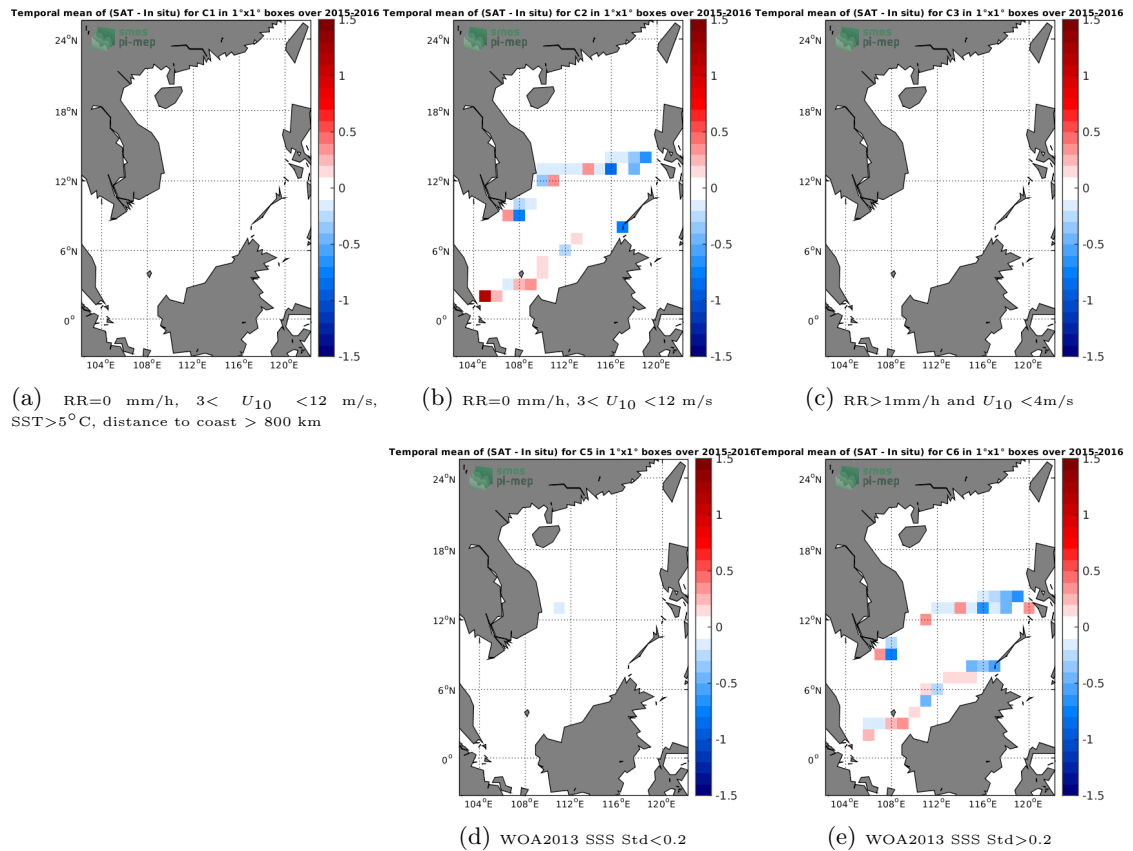
Figure 12: Temporal mean gridded over spatial boxes of size 1^\circ \times 1^\circ of \Delta SSS (SMOS-L3-CATDS-CPDC-V317-MONTHLY-25KM - TSG-SAMOS) for 5 different subdatasets corresponding to:RR=0 mm/h, 3 < U_{10} < 12 m/s, SST >5^\circ C, distance to coast > 800 km (a), RR=0 mm/h, 3 < U_{10} < 12 m/s (b), RR >1 mm/h and U_{10} < 4 m/s (c), WOA2013 SSS Std <0.2 (d), WOA2013 SSS Std >0.2 (e).
