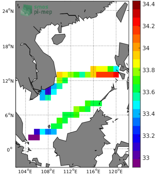
(c) MEAN(TSG-SAMOS SSS)
