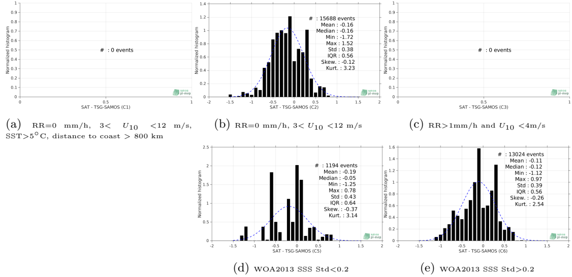
Figure 13: Normalized histogram of \Delta\text{SSS} (SMOS-L3-CATDS-CPDC-V317-MONTHLY-25KM - TSG-SAMOS) for 5 different subdatasets corresponding to: RR=0 mm/h, 3 < U_{10} < 12 m/s, SST > 5^{\circ}\text{C} , distance to coast > 800 km (a), RR=0 mm/h, 3 < U_{10} < 12 m/s (b), RR > 1\text{mm/h} and U_{10} < 4\text{m/s} (c), WOA2013 SSS Std < 0.2 (d), WOA2013 SSS Std > 0.2 (e).
