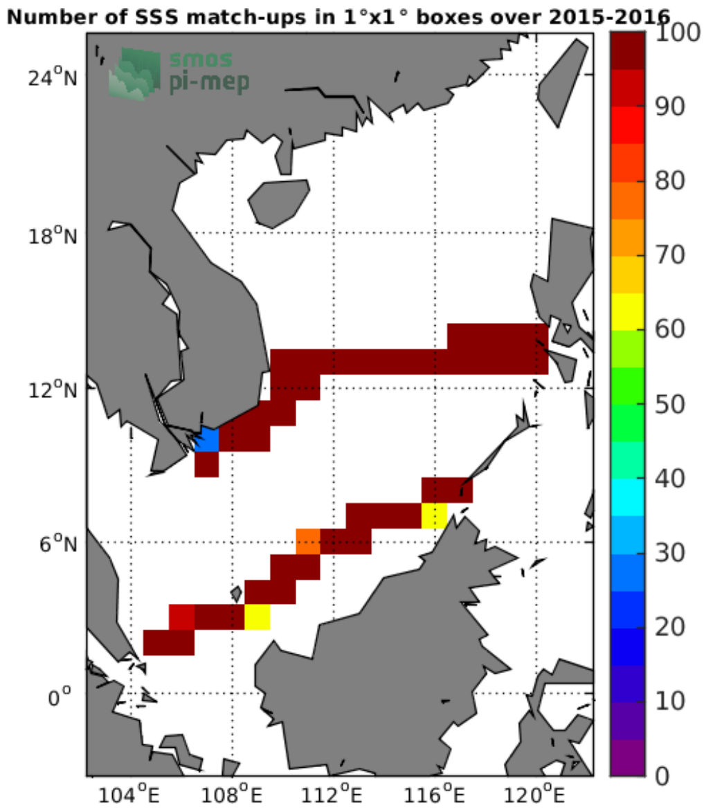
Figure 4: Number of SSS match-ups between TSG-SAMOS SSS and the SMOS-L3-CATDS-CPDC-V317-MONTHLY-25KM SSS product for the South China Sea Pi-MEP region over 1°x1° boxes and for the full satellite product period.
