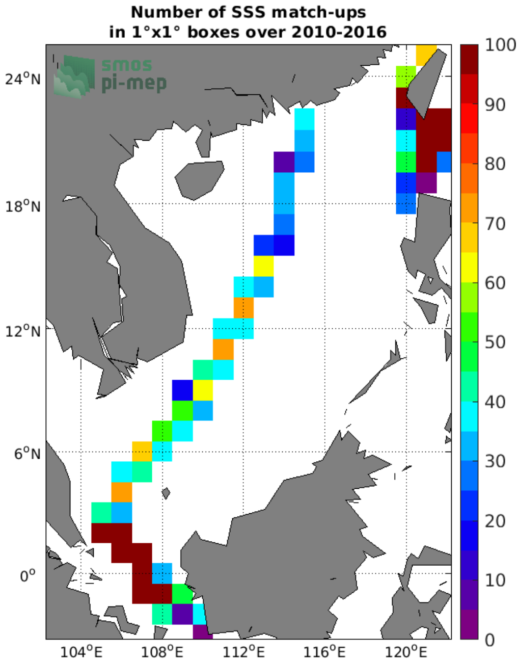
Figure 4: Number of SSS match-ups between TSG (LEGOS-DM) SSS and the SMOS SSS L3 v317 - Monthly - 25 km (CATDS-CPDC) SSS product for the South China Sea Pi-MEP region over 1°x1° boxes and for the full satellite product period.
