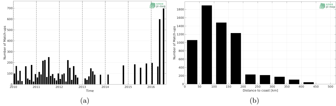
Figure 1: Number of match-ups between TSG-LEGOS-DM and SMOS L3 v317 - Monthly - 25 km (CATDS-CPDC) SSS as a function of time (a) and as function of the distance to coast (b) over the South China Sea Pi-MEP region and for the full satellite product period.
