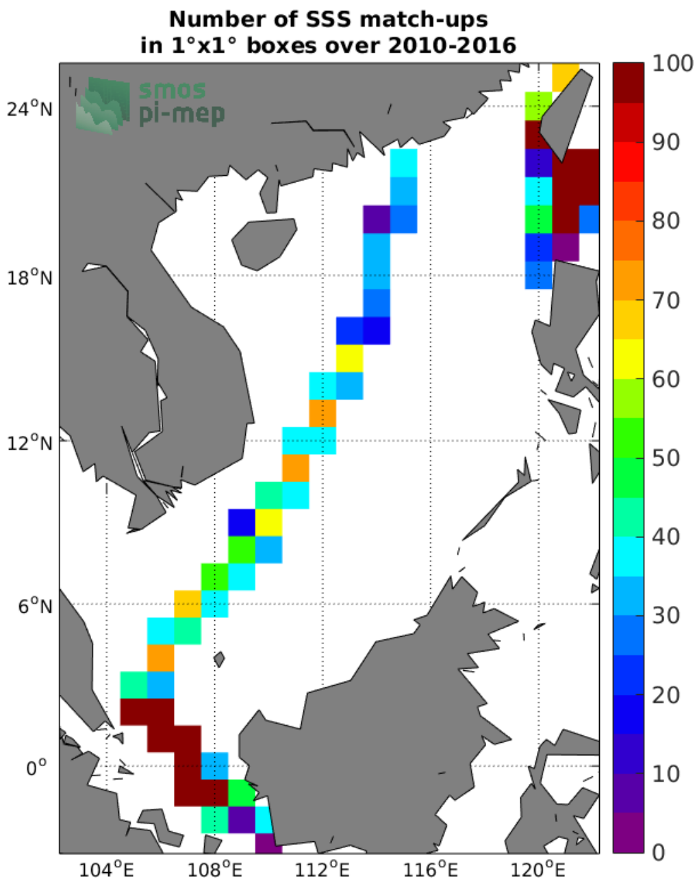
Figure 4: Number of SSS match-ups between TSG-LEGOS-DM SSS and the SMOS L3 v317 - Monthly - 25 km (CATDS-CPDC) SSS product for the South China Sea Pi-MEP region over 1°x1° boxes and for the full satellite product period.
