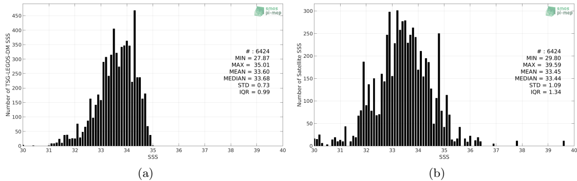
Figure 2: Histograms of SSS from TSG-LEGOS-DM (a) and SMOS L3 v317 - Monthly - 25 km (CATDS-CPDC) (b) considering all match-up pairs per bins of 0.1 over the South China Sea Pi-MEP region and for the full satellite product period.
