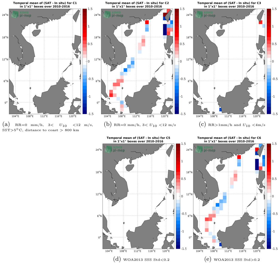
Figure 12: Temporal mean gridded over spatial boxes of size 1°x1° of \Delta SSS (SMOS L3 v317 - Monthly - 25 km (CATDS-CPDC) - TSG-LEGOS-DM) for 5 different subdatasets corresponding to:RR=0 mm/h, 3 < U_{10} < 12 m/s, SST>5°C, distance to coast > 800 km (a), RR=0 mm/h, 3 < U_{10} < 12 m/s (b), RR>1mm/h and U_{10} < 4 m/s (c), WOA2013 SSS Std<0.2 (d), WOA2013 SSS Std>0.2 (e).
