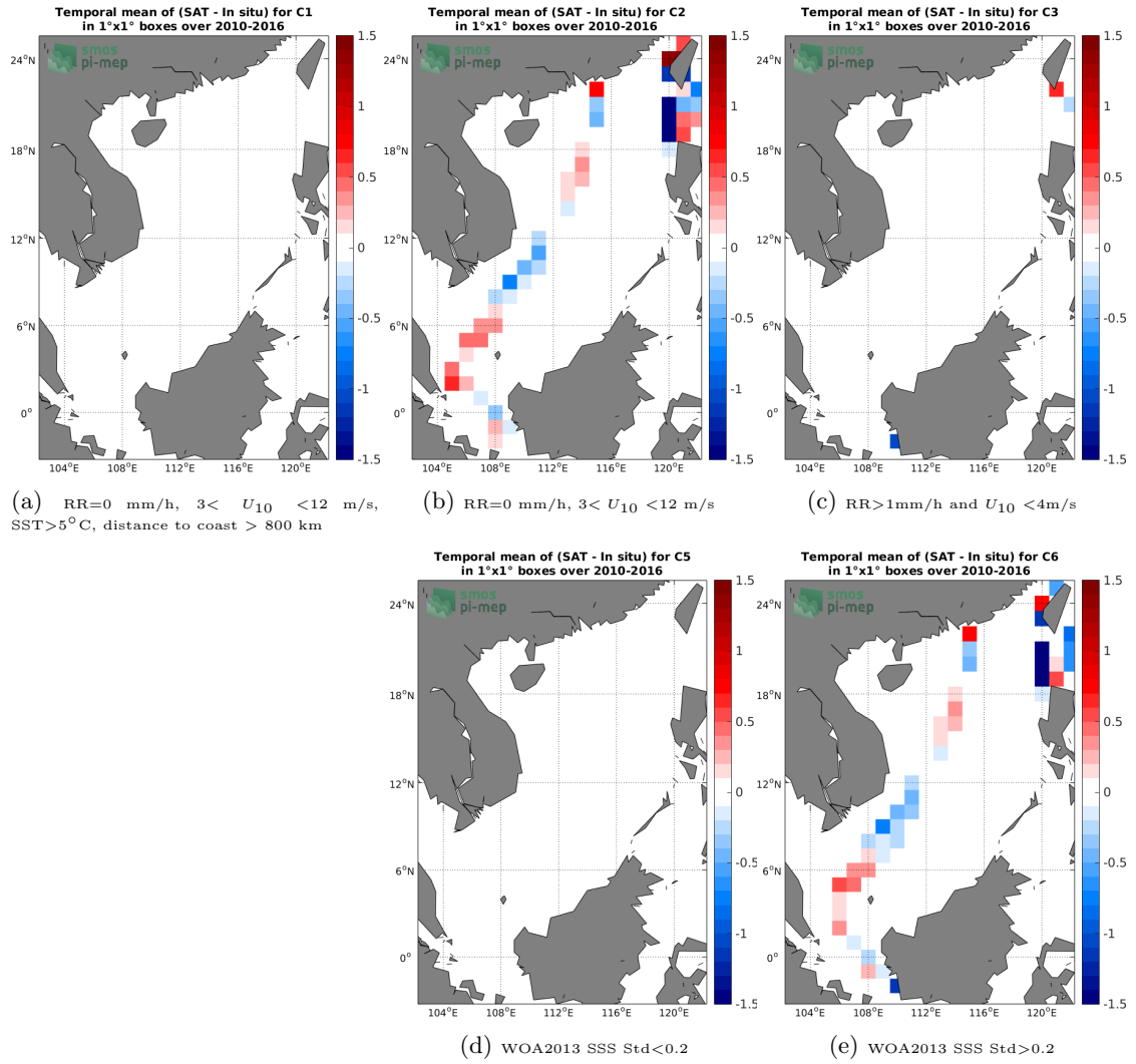
Figure 12: Temporal mean gridded over spatial boxes of size 1^\circ \times 1^\circ of \Delta SSS (SMOS-L3-CATDS-CPDC-V317-MONTHLY-25KM - TSG-LEGOS-DM) for 5 different subdatasets corresponding to: RR=0 mm/h, 3 < U_{10} < 12 m/s, SST > 5°C, distance to coast > 800 km (a), RR=0 mm/h, 3 < U_{10} < 12 m/s (b), RR > 1mm/h and U_{10} < 4 m/s (c), WOA2013 SSS Std < 0.2 (d), WOA2013 SSS Std > 0.2 (e).
