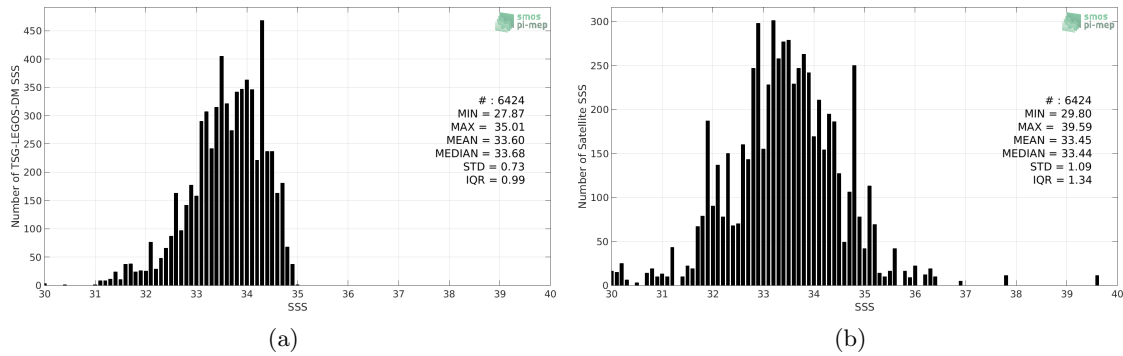
Figure 2: Histograms of SSS from TSG-LEGOS-DM (a) and SMOS-L3-CATDS-CPDC-V317-MONTHLY-25KM (b) considering all match-up pairs per bins of 0.1 over the South China Sea Pi-MEP region and for the full satellite product period.
