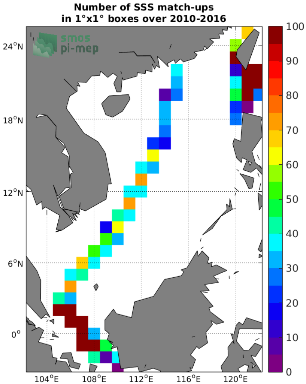
Figure 4: Number of SSS match-ups between TSG-LEGOS-DM SSS and the SMOS-L3-CATDS-CPDC-V317-MONTHLY-25KM SSS product for the South China Sea Pi-MEP region over 1°x1° boxes and for the full satellite product period.
