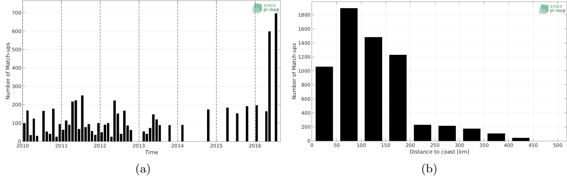
Figure 1: Number of match-ups between TSG-LEGOS-DM and SMOS-L3-CATDS-CPDC-V317-MONTHLY-25KM SSS as a function of time (a) and as function of the distance to coast (b) over the South China Sea Pi-MEP region and for the full satellite product period.
