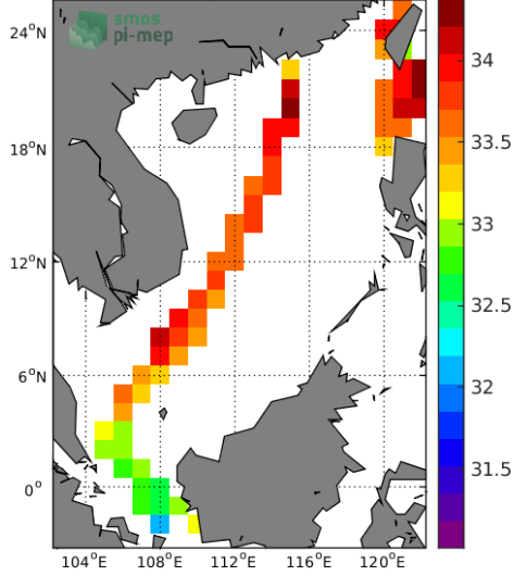
(c) MEAN(TSG-LEGOS-DM SSS)
