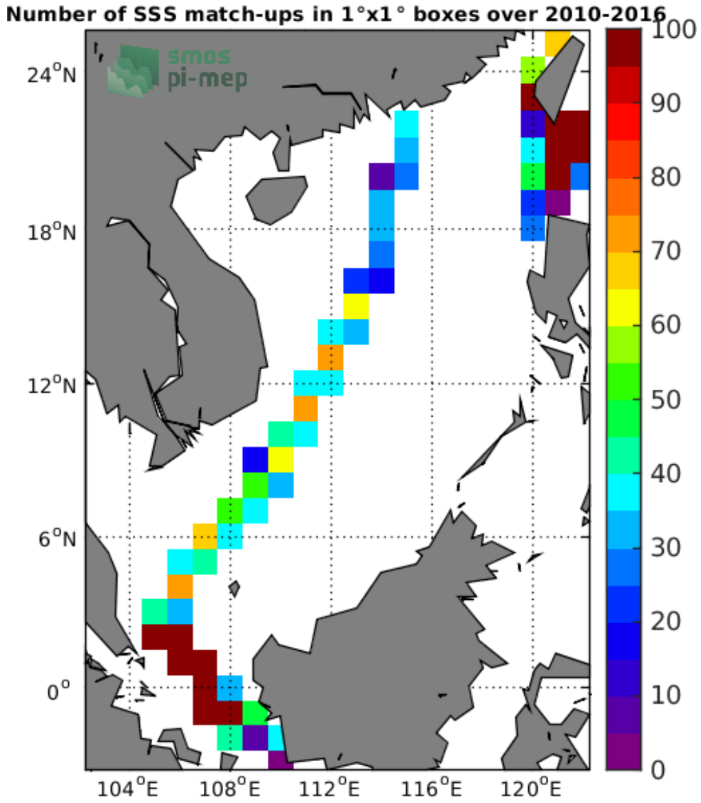
Figure 4: Number of SSS match-ups between TSG-LEGOS-DM SSS and the SMOS-L3-CATDS-CPDC-V317-MONTHLY-25KM SSS product for the South China Sea Pi-MEP region over 1°x1° boxes and for the full satellite product period.
