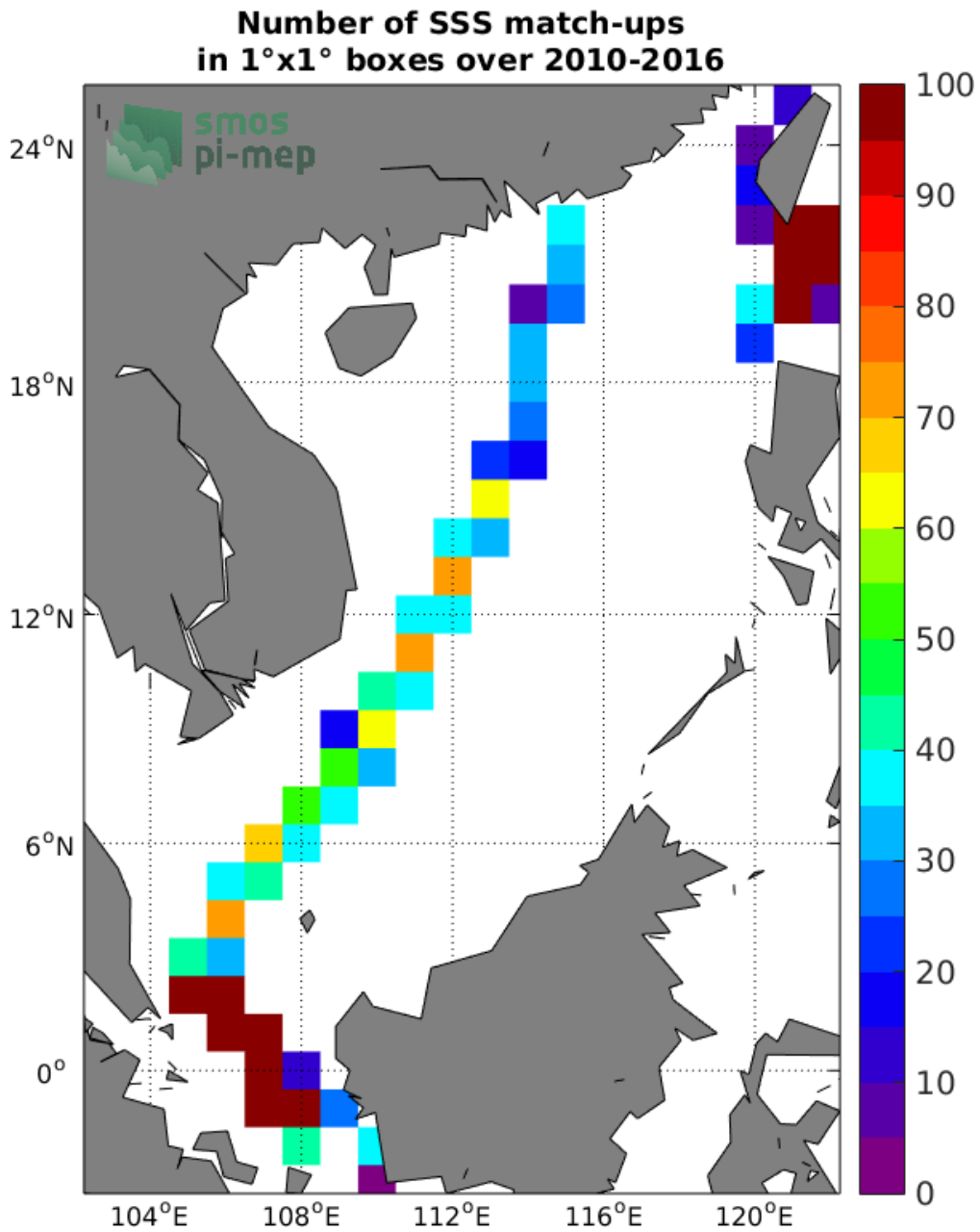
Figure 4: Number of SSS match-ups between TSG-LEGOS-DM SSS and the SMOS L3 v317 - 10 Days - 25 km (CATDS-CPDC) SSS product for the South China Sea Pi-MEP region over 1°x1° boxes and for the full satellite product period.
