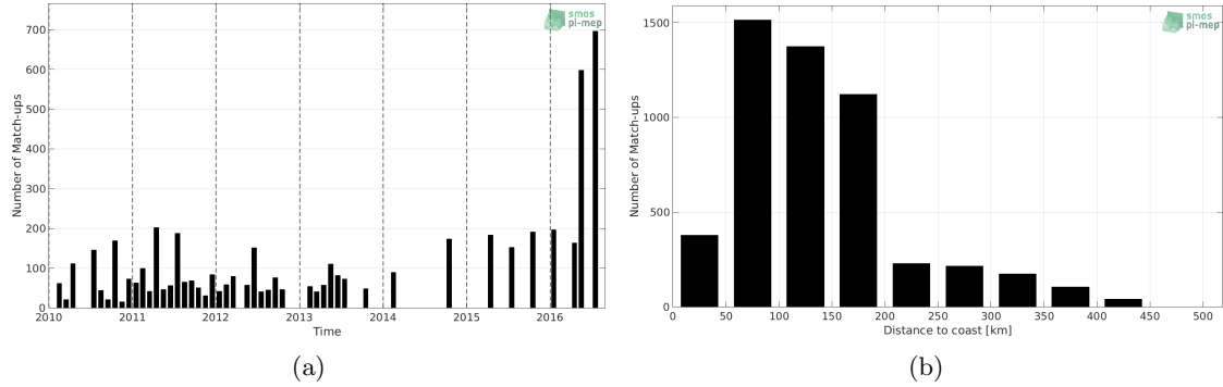
Figure 1: Number of match-ups between TSG-LEGOS-DM and SMOS L3 v317 - 10 Days - 25 km (CATDS-CPDC) SSS as a function of time (a) and as function of the distance to coast (b) over the South China Sea Pi-MEP region and for the full satellite product period.
