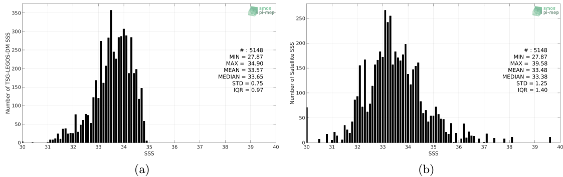
Figure 2: Histograms of SSS from TSG-LEGOS-DM (a) and SMOS L3 v317 - 10 Days - 25 km (CATDS-CPDC) (b) considering all match-up pairs per bins of 0.1 over the South China Sea Pi-MEP region and for the full satellite product period.
