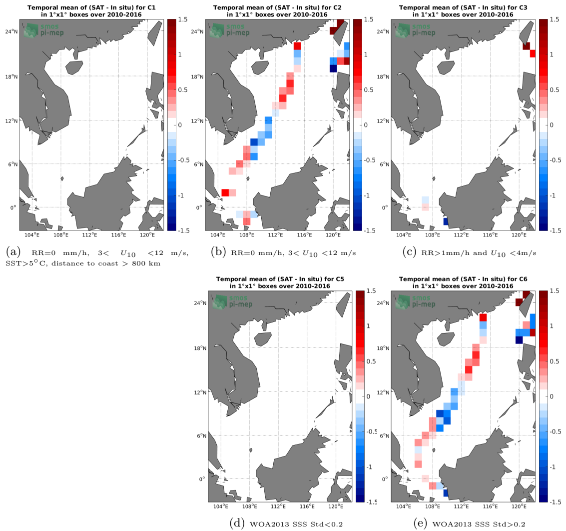
Figure 12: Temporal mean gridded over spatial boxes of size 1^\circ \times 1^\circ of \Delta SSS (SMOS L3 v317 - 10 Days - 25 km (CATDS-CPDC) - TSG-LEGOS-DM) for 5 different subdatasets corresponding to: RR=0 mm/h, 3 < U_{10} < 12 m/s, SST>5°C, distance to coast > 800 km (a), RR=0 mm/h, 3 < U_{10} < 12 m/s (b), RR>1mm/h and U_{10} < 4 m/s (c), WOA2013 SSS Std<0.2 (d), WOA2013 SSS Std>0.2 (e).
