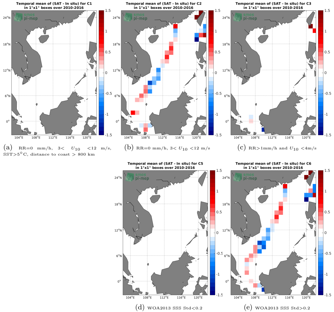
Figure 12: Temporal mean gridded over spatial boxes of size 1^\circ \times 1^\circ of \Delta SSS (SMOS-L3-CATDS-CPDC-V317-10DAYS-25KM - TSG-LEGOS-DM) for 5 different subdatasets corresponding to:RR=0 mm/h, 3 < U_{10} < 12 m/s, SST>5°C, distance to coast > 800 km (a), RR=0 mm/h, 3 < U_{10} < 12 m/s (b), RR>1mm/h and U_{10} < 4 m/s (c), WOA2013 SSS Std<0.2 (d), WOA2013 SSS Std>0.2 (e).
