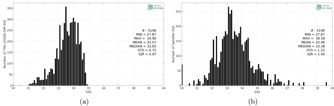
Figure 2: Histograms of SSS from TSG-LEGOS-DM (a) and SMOS-L3-CATDS-CPDC-V317-10DAYS-25KM (b) considering all match-up pairs per bins of 0.1 over the South China Sea Pi-MEP region and for the full satellite product period.
