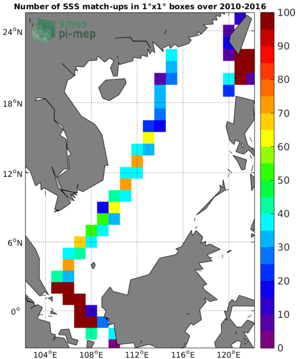
Figure 4: Number of SSS match-ups between TSG-LEGOS-DM SSS and the SMOS-L3-CATDS-CPDC-V317-10DAYS-25KM SSS product for the South China Sea Pi-MEP region over 1°x1° boxes and for the full satellite product period.
