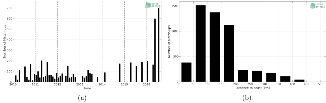
Figure 1: Number of match-ups between TSG-LEGOS-DM and SMOS-L3-CATDS-CPDC-V317-10DAYS-25KM SSS as a function of time (a) and as function of the distance to coast (b) over the South China Sea Pi-MEP region and for the full satellite product period.
