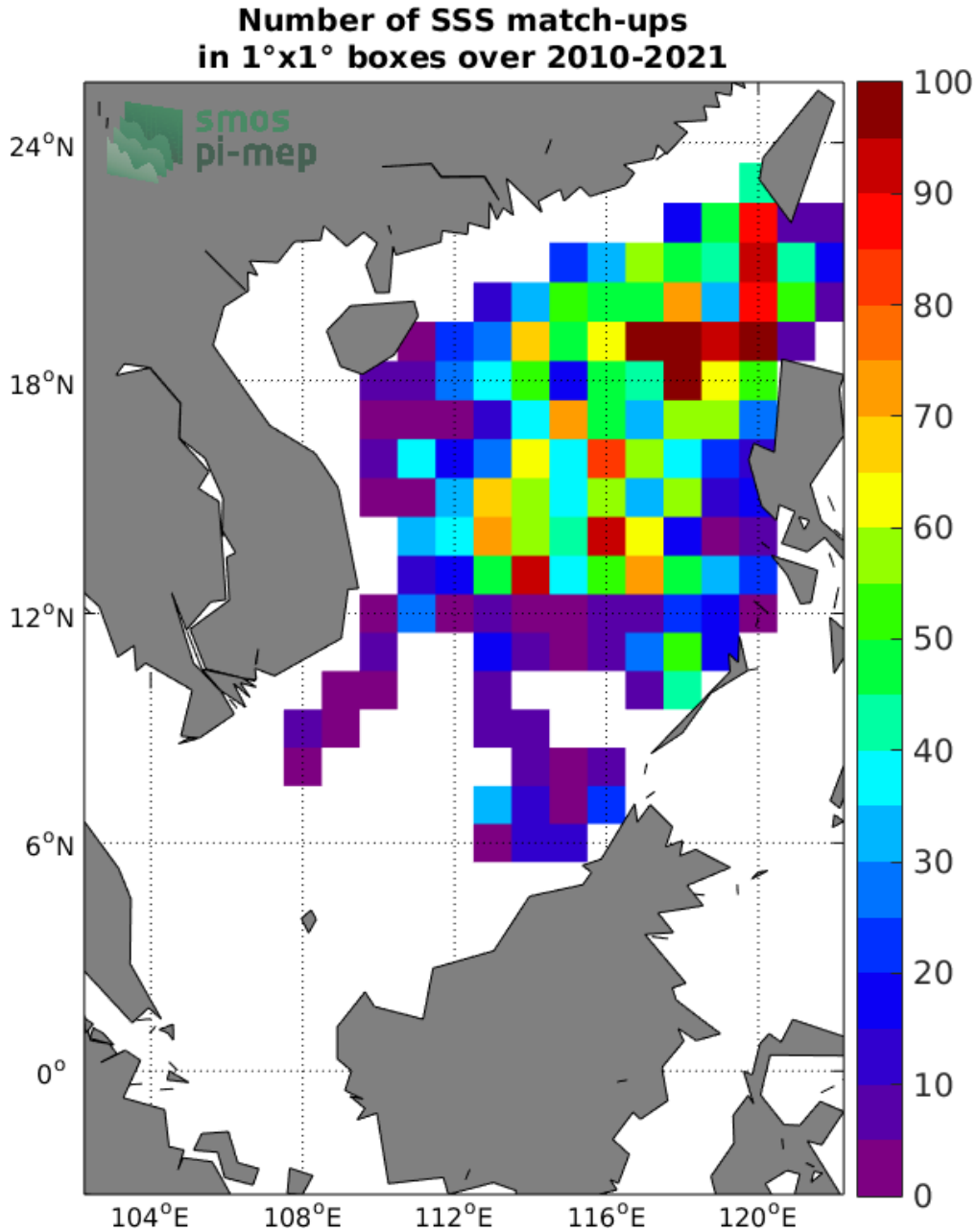
Figure 4: Number of SSS match-ups between Argo SSS and the SMOS SSS L3 v317 - 10 Days - 25 km (CATDS-CPDC) SSS product for the South China Sea Pi-MEP region over 1^\circ \times 1^\circ boxes and for the full satellite product period.
