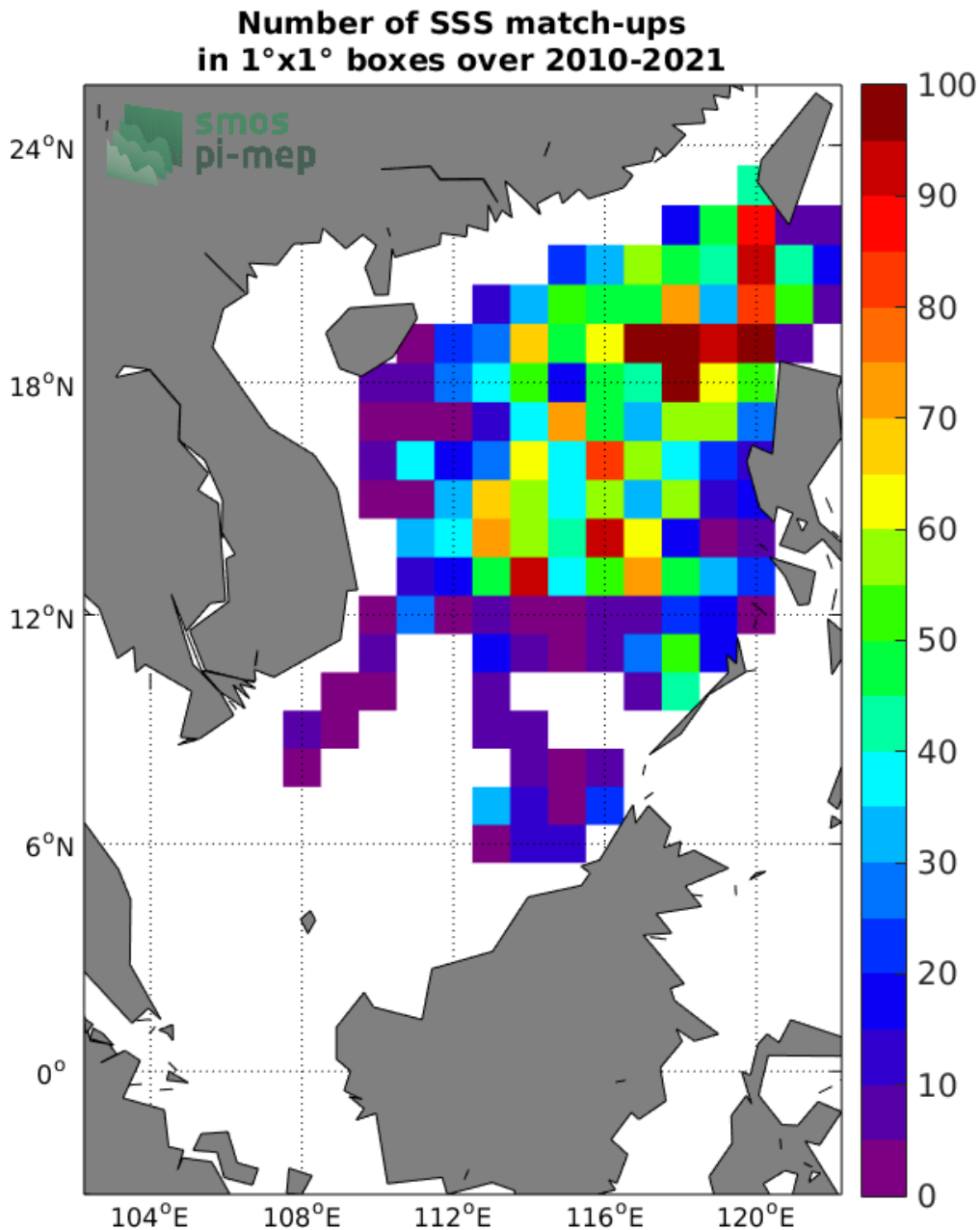
Figure 4: Number of SSS match-ups between Argo SSS and the SMOS SSS L3 v317 - 10 Days - 25 km (CATDS-CPDC) SSS product for the South China Sea Pi-MEP region over 1°x1° boxes and for the full satellite product period.
