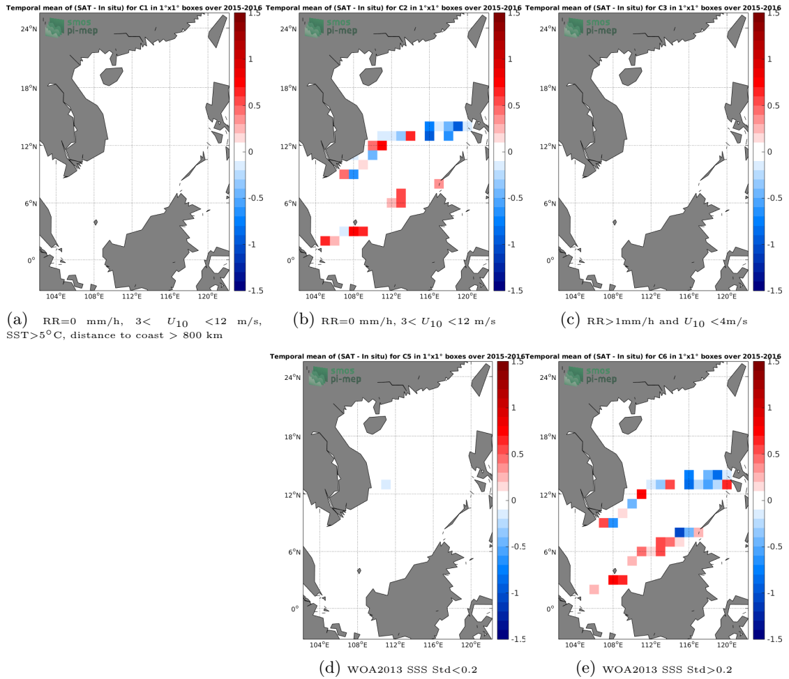
Figure 12: Temporal mean gridded over spatial boxes of size 1^\circ \times 1^\circ of \Delta SSS (SMOS-L3-CATDS-CPDC-V3-10DAYS-25KM - TSG-SAMOS) for 5 different subdatasets corresponding to: RR=0 mm/h, 3 < U_{10} < 12 m/s, SST > 5^\circ C , distance to coast > 800 km (a), RR=0 mm/h, 3 < U_{10} < 12 m/s (b), RR > 1 mm/h and U_{10} < 4 m/s (c), WOA2013 SSS Std < 0.2 (d), WOA2013 SSS Std > 0.2 (e).
