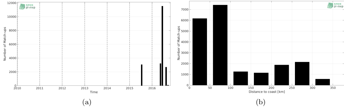
Figure 1: Number of match-ups between TSG-SAMOS and SMOS-L3-CATDS-CPDC-V3-10DAYS-25KM SSS as a function of time (a) and as function of the distance to coast (b) over the South China Sea Pi-MEP region and for the full satellite product period.
