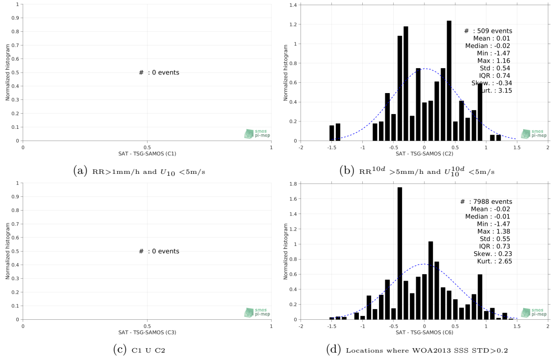
Figure 13: Normalized histogram of \Delta\text{SSS} (SMOS-L3-CATDS-CPDC-V3-10DAYS-25KM - TSG-SAMOS) for 6 different subdatasets corresponding to: RR > 1\text{mm/h} and U_{10} < 5\text{m/s} (a), RR^{10d} > 5\text{mm/h} and U_{10}^{10d} < 5\text{m/s} (b), C1 \cup C2 (c), Locations where WOA2013 SSS STD > 0.2 (d).
