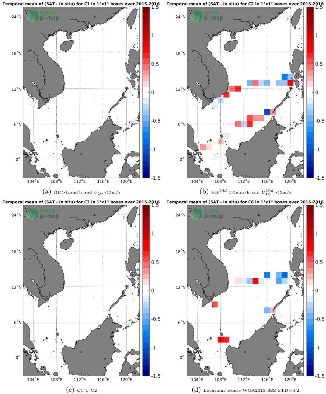
Figure 12: Temporal mean gridded over spatial boxes of size 1°x1° of \Delta\text{SSS} (SMOS-L3-CATDS-CPDC-V3-10DAYS-25KM - TSG-SAMOS) for 4 different subdatasets corresponding to: RR > 1\text{mm/h} and U_{10} < 5\text{m/s} (a), RR^{10d} > 5\text{mm/h} and U_{10}^{10d} < 5\text{m/s} (b), C1 U C2 (c), Locations where WOA2013 SSS STD > 0.2 (d).
