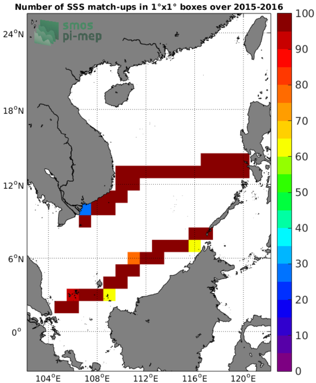
Figure 4: Number of SSS match-ups between TSG-SAMOS SSS and the SMOS-L3-CATDS-CPDC-V3-10DAYS-25KM SSS product for the South China Sea Pi-MEP region over 1°x1° boxes and for the full satellite product period.
