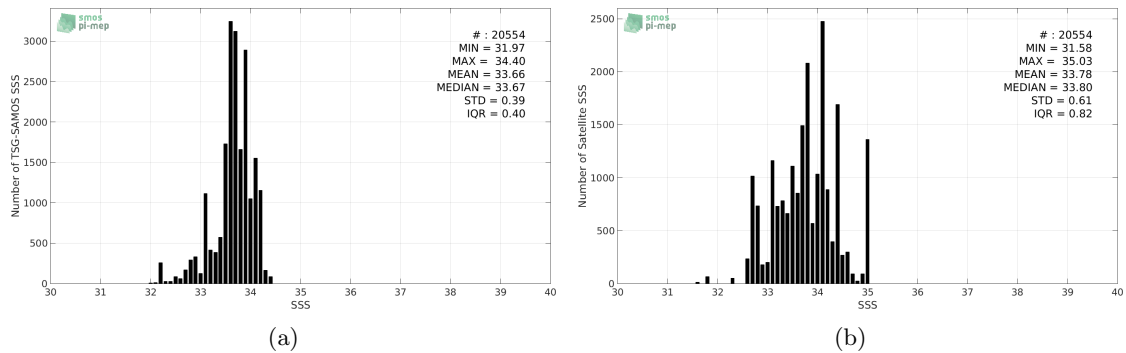
Figure 2: Histograms of SSS from TSG-SAMOS (a) and SMOS-L3-CATDS-CPDC-V3-10DAYS-25KM (b) considering all match-up pairs per bins of 0.1 over the South China Sea Pi-MEP region and for the full satellite product period.
