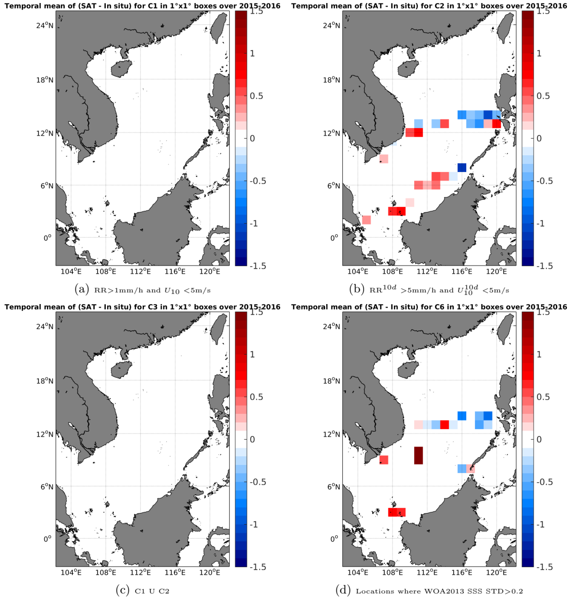
Figure 12: Temporal mean gridded over spatial boxes of size 1°x1° of \Delta SSS (SMOS-L3-CATDS-CPDC-V3-10DAYS-25KM - TSG-SAMOS) for 4 different subdatasets corresponding to: RR > 1\text{mm/h} and U_{10} < 5\text{m/s} (a), RR^{10d} > 5\text{mm/h} and U_{10}^{10d} < 5\text{m/s} (b), C1 U C2 (c), Locations where WOA2013 SSS STD > 0.2 (d).
