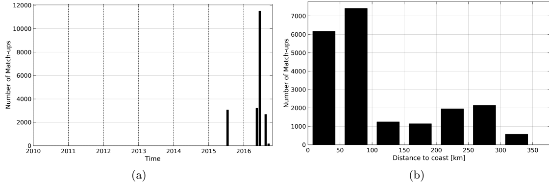
Figure 1: Number of match-ups between TSG-SAMOS and SMOS-L3-CATDS-CPDC-V3-10DAYS-25KM SSS as a function of time (a) and as function of the distance to coast (b) over the South China Sea Pi-MEP region and for the full satellite product period.
