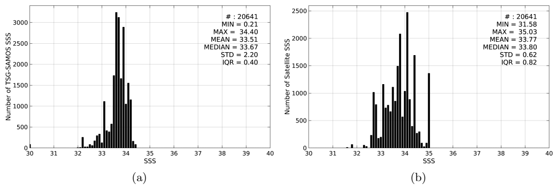
Figure 2: Histograms of SSS from TSG-SAMOS (a) and SMOS-L3-CATDS-CPDC-V3-10DAYS-25KM (b) considering all match-up pairs per bins of 0.1 over the South China Sea Pi-MEP region and for the full satellite product period.
