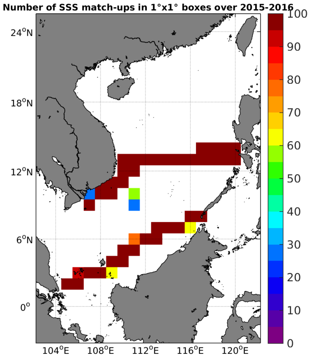
Figure 4: Number of SSS match-ups between TSG-SAMOS SSS and the SMOS-L3-CATDS-CPDC-V3-10DAYS-25KM SSS product for the South China Sea Pi-MEP region over 1°x1° boxes and for the full satellite product period.
