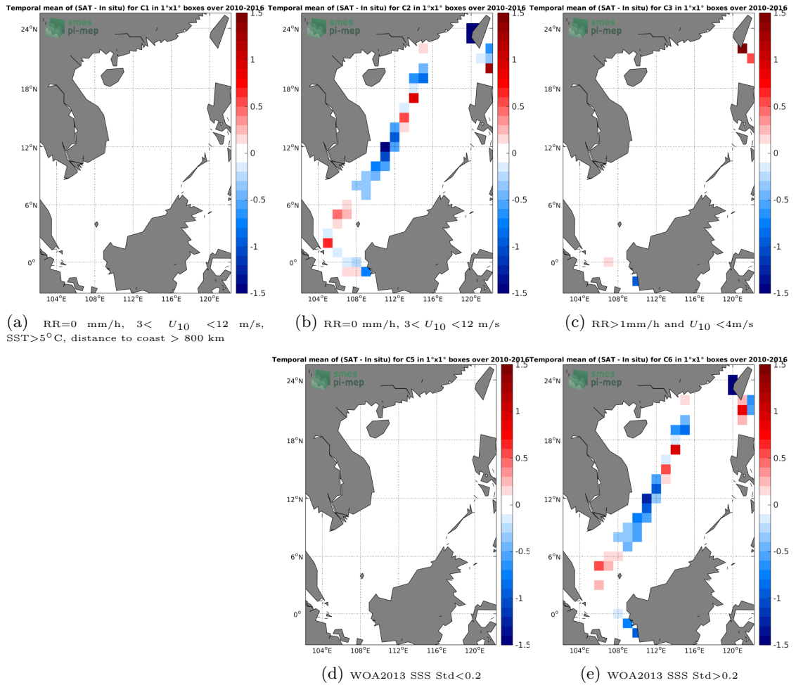
Figure 12: Temporal mean gridded over spatial boxes of size 1^\circ \times 1^\circ of \Delta SSS (SMOS-L3-CATDS-CPDC-V3-10DAYS-25KM - TSG-LEGOS-DM) for 5 different subdatasets corresponding to:RR=0 mm/h, 3 < U_{10} < 12 m/s, SST >5^\circ C, distance to coast > 800 km (a), RR=0 mm/h, 3 < U_{10} < 12 m/s (b), RR >1 mm/h and U_{10} < 4 m/s (c), WOA2013 SSS Std <0.2 (d), WOA2013 SSS Std >0.2 (e).
