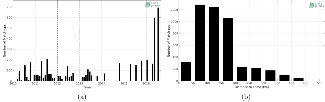
Figure 1: Number of match-ups between TSG-LEGOS-DM and SMOS-L3-CATDS-CPDC-V3-10DAYS-25KM SSS as a function of time (a) and as function of the distance to coast (b) over the South China Sea Pi-MEP region and for the full satellite product period.
