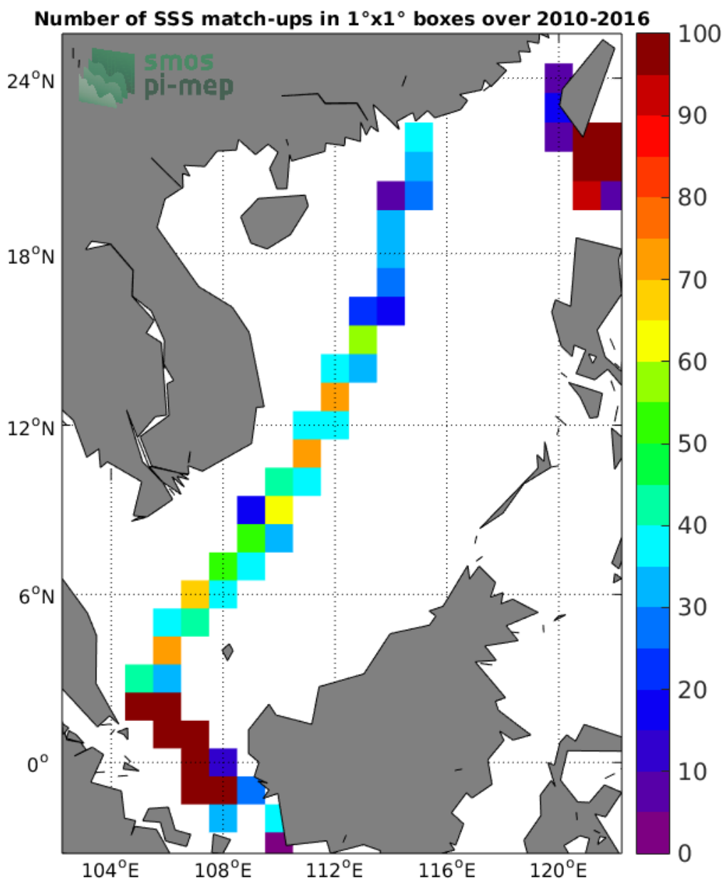
Figure 4: Number of SSS match-ups between TSG-LEGOS-DM SSS and the SMOS-L3-CATDS-CPDC-V3-10DAYS-25KM SSS product for the South China Sea Pi-MEP region over 1°x1° boxes and for the full satellite product period.
