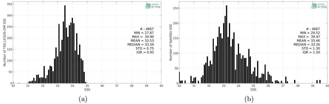
Figure 2: Histograms of SSS from TSG-LEGOS-DM (a) and SMOS-L3-CATDS-CPDC-V3-10DAYS-25KM (b) considering all match-up pairs per bins of 0.1 over the South China Sea Pi-MEP region and for the full satellite product period.
