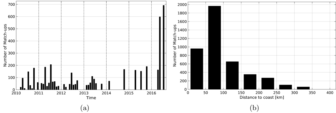
Figure 1: Number of match-ups between TSG-LEGOS-DM and SMOS-L3-CATDS-CPDC-V3-10DAYS-25KM SSS as a function of time (a) and as function of the distance to coast (b) over the South China Sea Pi-MEP region and for the full satellite product period.
