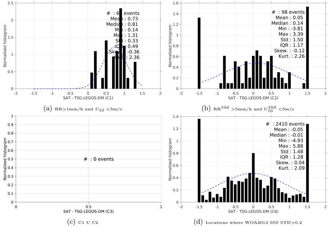
Figure 13: Normalized histogram of \Delta\text{SSS} (SMOS-L3-CATDS-CPDC-V3-10DAYS-25KM - TSG-LEGOS-DM) for 6 different subdatasets corresponding to: RR > 1mm/h and U_{10} < 5\text{m/s} (a), RR^{10d} > 5\text{mm/h} and U_{10}^{10d} < 5\text{m/s} (b), C1 U C2 (c), Locations where WOA2013 SSS STD > 0.2 (d).
