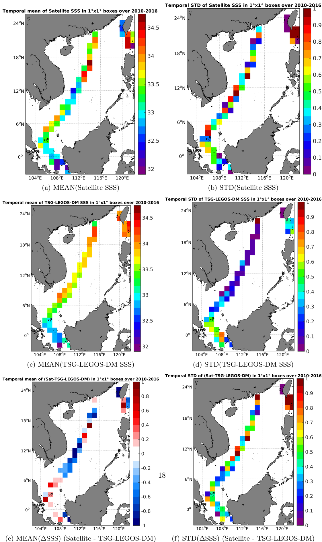
Figure 6: Temporal mean (left) and STD (right) of SSS from SMOS-L3-CATDS-CPDC-V3-10DAYS-25KM (top), TSG-LEGOS-DM (middle), and of \Delta SSS (Satellite - TSG-LEGOS-DM). Only match-up pairs are used to generate these maps.
