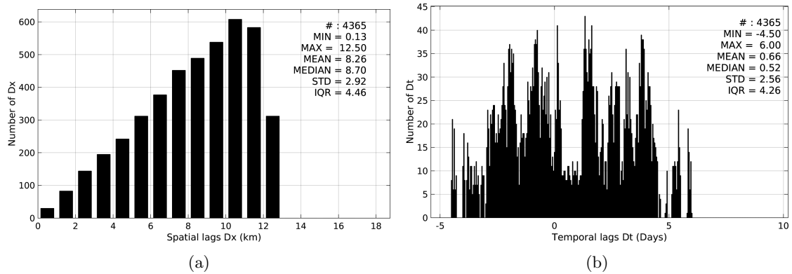
Figure 5: Histograms of the spatial (a) and temporal (b) lags between the time of the TSG-LEGOS-DM measurements and the date of the corresponding SMOS-L3-CATDS-CPDC-V3-10DAYS-25KM SSS product.
