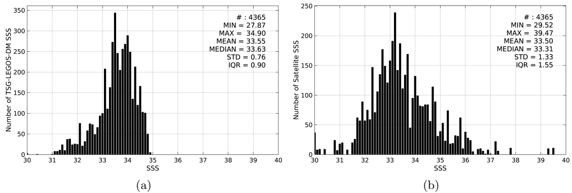
Figure 2: Histograms of SSS from TSG-LEGOS-DM (a) and SMOS-L3-CATDS-CPDC-V3-10DAYS-25KM (b) considering all match-up pairs per bins of 0.1 over the South China Sea Pi-MEP region and for the full satellite product period.
