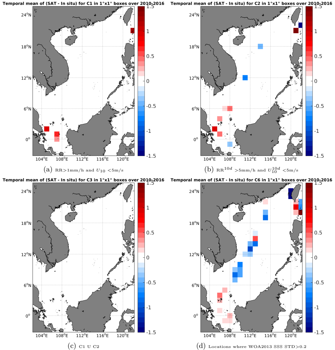
Figure 12: Temporal mean gridded over spatial boxes of size 1°x1° of \Delta SSS (SMOS-L3-CATDS-CPDC-V3-10DAYS-25KM - TSG-LEGOS-DM) for 4 different subdatasets corresponding to:RR>1mm/h and U_{10} < 5 m/s (a), RR^{10d} > 5 mm/h and U_{10}^{10d} < 5 m/s (b), C1 U C2 (c),Locations where WOA2013 SSS STD>0.2 (d).
