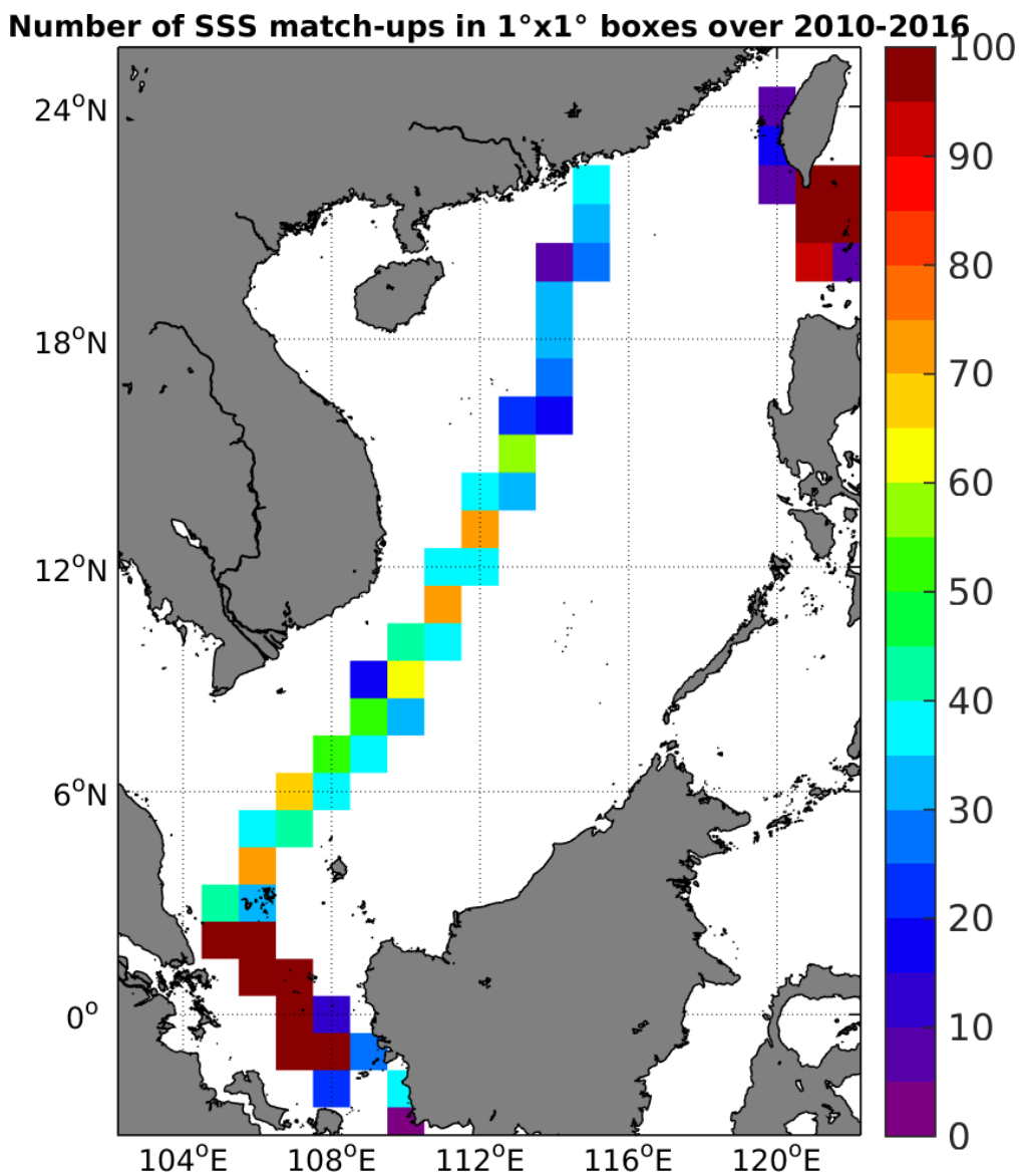
Figure 4: Number of SSS match-ups between TSG-LEGOS-DM SSS and the SMOS-L3-CATDS-CPDC-V3-10DAYS-25KM SSS product for the South China Sea Pi-MEP region over 1°x1° boxes and for the full satellite product period.
