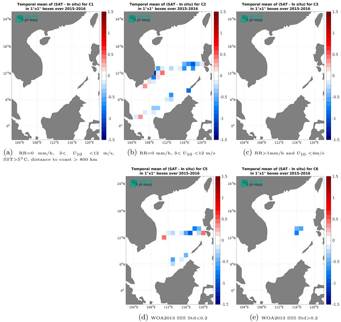
Figure 12: Temporal mean gridded over spatial boxes of size 1^\circ \times 1^\circ of \Delta\text{SSS} (SMOS SSS L3 v2 - 9-Days (BEC) - TSG (SAMOS)) for 5 different subdatasets corresponding to:RR=0 mm/h, 3 < U_{10} < 12 m/s, SST>5°C, distance to coast > 800 km (a), RR=0 mm/h, 3 < U_{10} < 12 m/s (b), RR>1mm/h and U_{10} < 4 m/s (c), WOA2013 SSS Std<0.2 (d), WOA2013 SSS Std>0.2 (e).
