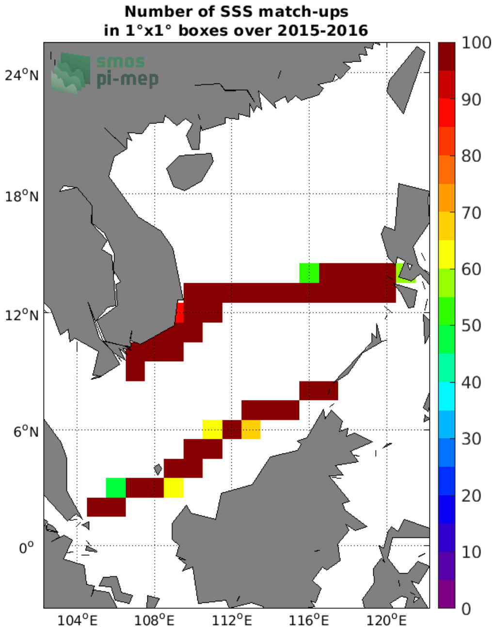
Figure 4: Number of SSS match-ups between TSG (SAMOS) SSS and the SMOS SSS L3 v2 - 9-Days (BEC) SSS product for the South China Sea Pi-MEP region over 1°x1° boxes and for the full satellite product period.
