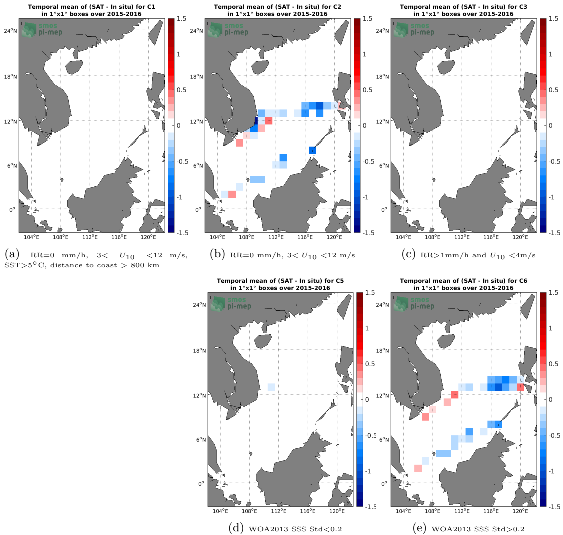
Figure 12: Temporal mean gridded over spatial boxes of size 1°x1° of \Delta SSS (SMOS SSS L3 v2 - 9-Days (BEC) - TSG (SAMOS)) for 5 different subdatasets corresponding to:RR=0 mm/h, 3 < U_{10} < 12 m/s, SST > 5°C, distance to coast > 800 km (a), RR=0 mm/h, 3 < U_{10} < 12 m/s (b), RR > 1mm/h and U_{10} < 4m/s (c), WOA2013 SSS Std < 0.2 (d), WOA2013 SSS Std > 0.2 (e).
