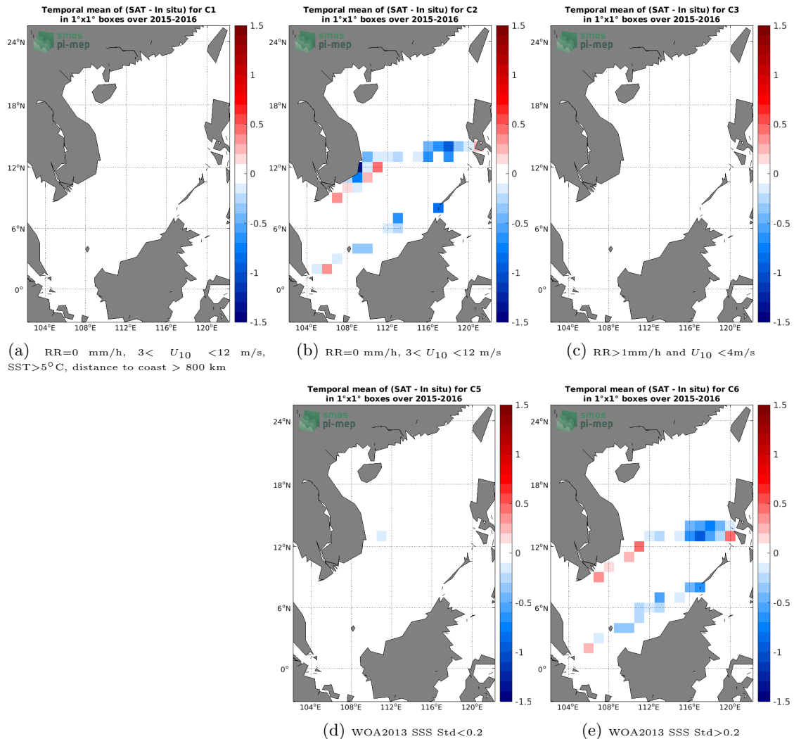
Figure 12: Temporal mean gridded over spatial boxes of size 1^\circ \times 1^\circ of \Delta SSS (SMOS SSS L3 v2 - 9-Days (BEC) - TSG (SAMOS)) for 5 different subdatasets corresponding to:RR=0 mm/h, 3 < U_{10} < 12 m/s, SST >5^\circ\text{C} , distance to coast > 800 km (a), RR=0 mm/h, 3 < U_{10} < 12 m/s (b), RR >1 mm/h and U_{10} < 4 m/s (c), WOA2013 SSS Std <0.2 (d), WOA2013 SSS Std >0.2 (e).
