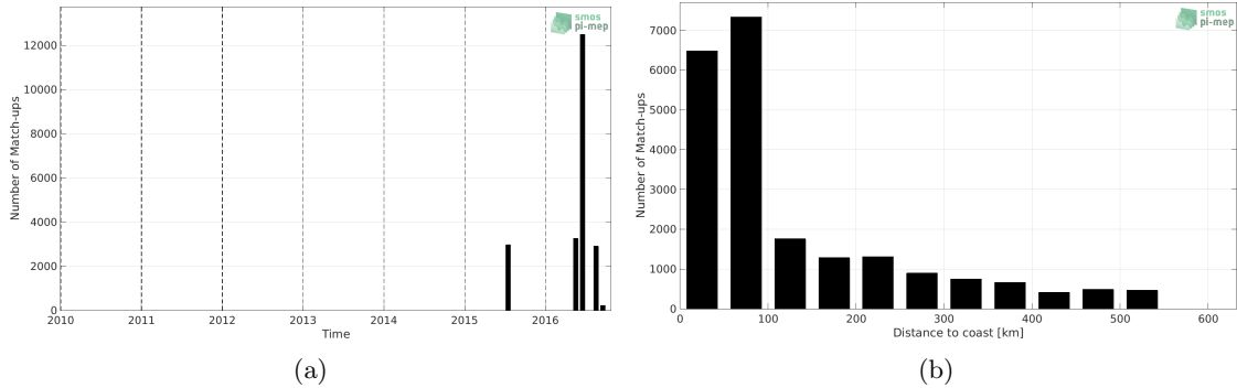
Figure 1: Number of match-ups between TSG (SAMOS) and SMOS SSS L3 v2 - 9-Days (BEC) SSS as a function of time (a) and as function of the distance to coast (b) over the South China Sea Pi-MEP region and for the full satellite product period.
