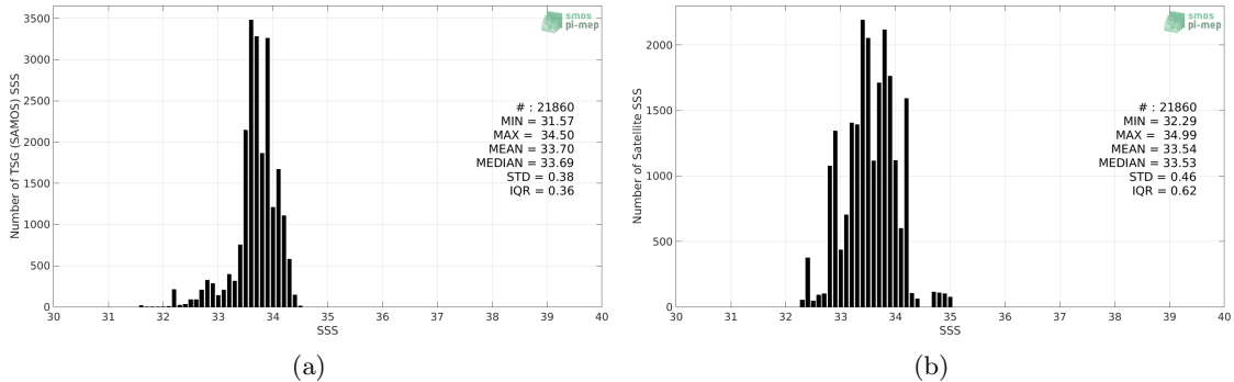
Figure 2: Histograms of SSS from TSG (SAMOS) (a) and SMOS SSS L3 v2 - 9-Days (BEC) (b) considering all match-up pairs per bins of 0.1 over the South China Sea Pi-MEP region and for the full satellite product period.
