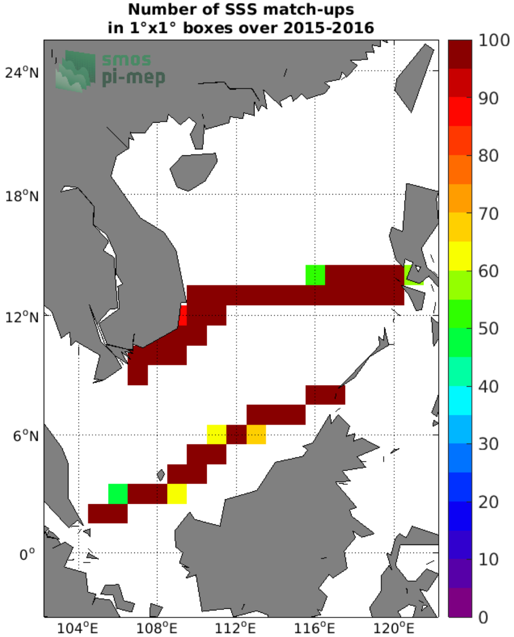
Figure 4: Number of SSS match-ups between TSG (SAMOS) SSS and the SMOS SSS L3 v2 - 9-Days (BEC) SSS product for the South China Sea Pi-MEP region over 1°x1° boxes and for the full satellite product period.
