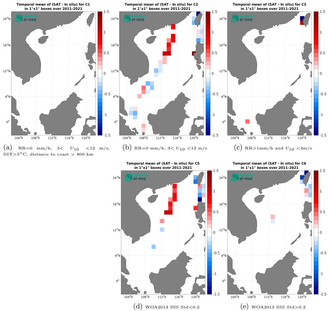
Figure 14: Temporal mean gridded over spatial boxes of size 1^{\circ} \times 1^{\circ} of \Delta SSS (SMOS SSS L3 v2 - 9-Days (BEC) - TSG (LEGOS-DM)) for 5 different subdatasets corresponding to:RR=0 mm/h, 3 < U_{10} < 12 m/s, SST>5°C, distance to coast > 800 km (a), RR=0 mm/h, 3 < U_{10} < 12 m/s (b), RR>1mm/h and U_{10} < 4 m/s (c), WOA2013 SSS Std<0.2 (d), WOA2013 SSS Std>0.2 (e).
