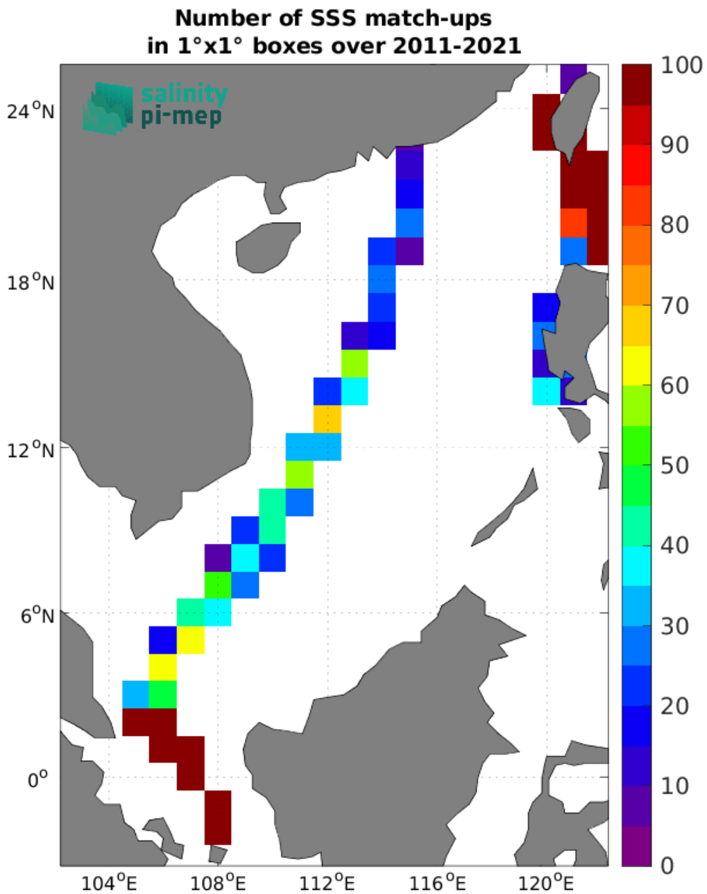
Figure 5: Number of SSS match-ups between TSG (LEGOS-DM) SSS and the SMOS SSS L3 v2 - 9-Days (BEC) SSS product for the South China Sea Pi-MEP region over 1^{\circ} \times 1^{\circ} boxes and for the full satellite product period.
