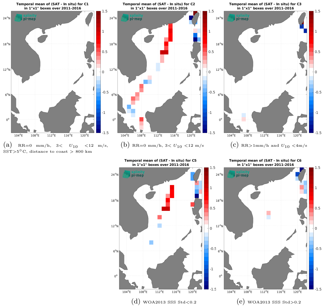
Figure 12: Temporal mean gridded over spatial boxes of size 1^\circ \times 1^\circ of \Delta\text{SSS} (SMOS SSS L3 v2 - 9-Days (BEC) - TSG (LEGOS-DM)) for 5 different subdatasets corresponding to:RR=0 mm/h, 3 < U_{10} < 12 m/s, SST >5^\circ\text{C} , distance to coast > 800 km (a), RR=0 mm/h, 3 < U_{10} < 12 m/s (b), RR >1 mm/h and U_{10} < 4 m/s (c), WOA2013 SSS Std <0.2 (d), WOA2013 SSS Std >0.2 (e).
