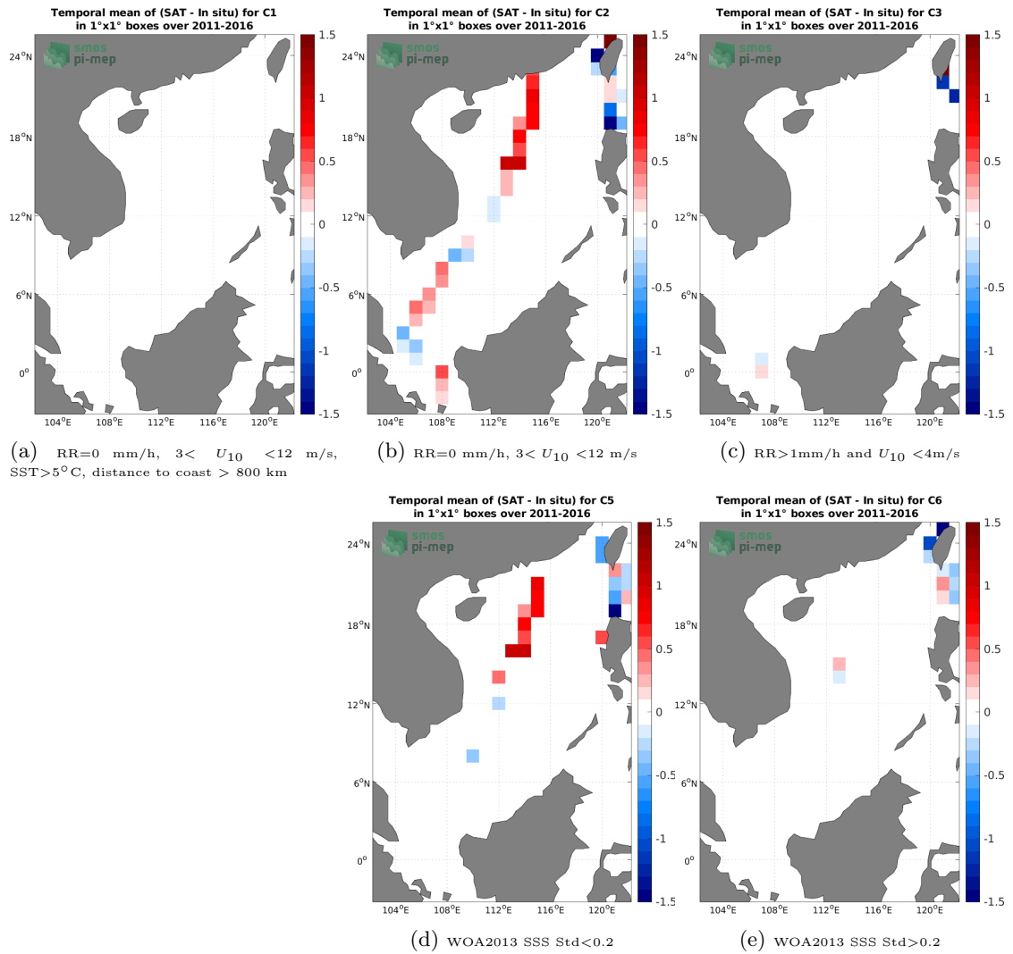
Figure 12: Temporal mean gridded over spatial boxes of size 1^\circ \times 1^\circ of \Delta SSS (SMOS SSS L3 v2 - 9-Days (BEC) - TSG (LEGOS-DM)) for 5 different subdatasets corresponding to:RR=0 mm/h, 3 < U_{10} < 12 m/s, SST>5°C, distance to coast > 800 km (a), RR=0 mm/h, 3 < U_{10} < 12 m/s (b), RR>1mm/h and U_{10} < 4 m/s (c), WOA2013 SSS Std<0.2 (d), WOA2013 SSS Std>0.2 (e).
