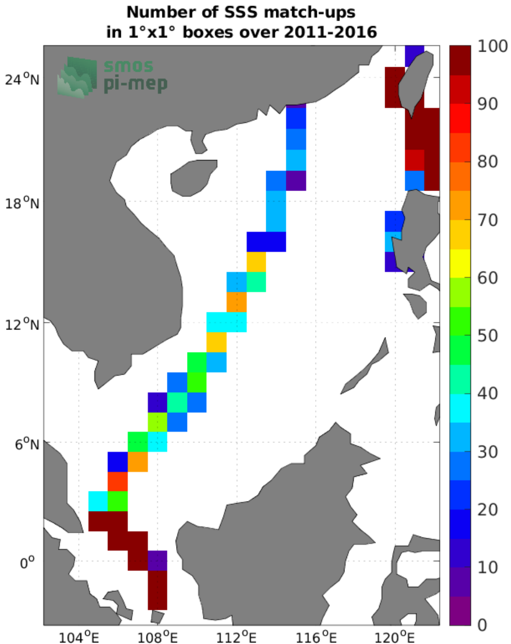
Figure 4: Number of SSS match-ups between TSG (LEGOS-DM) SSS and the SMOS SSS L3 v2 - 9-Days (BEC) SSS product for the South China Sea Pi-MEP region over 1°x1° boxes and for the full satellite product period.
