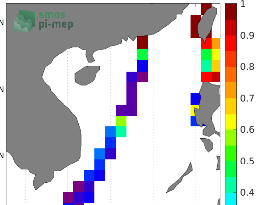
Temporal STD of (Sat - TSG (LEGOS-DM)) in 1°x1° boxes over 2011-2016
