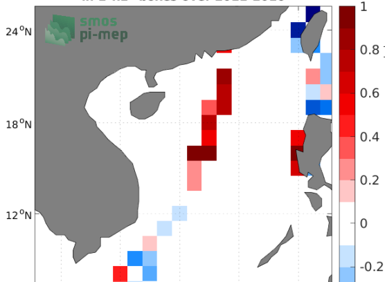
Temporal mean of (Sat - TSG (LEGOS-DM)) in 1°x1° boxes over 2011-2016
