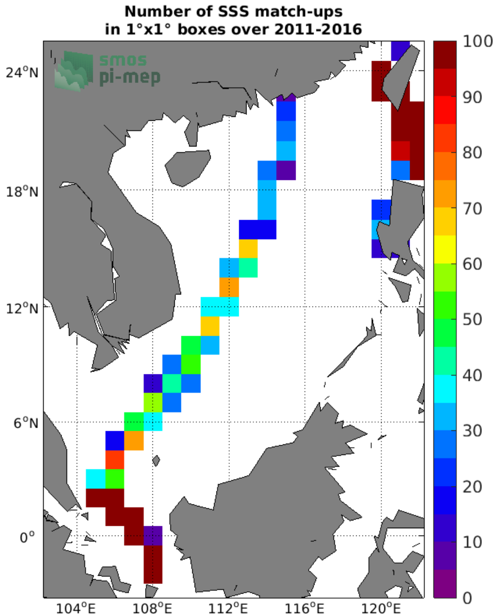
Figure 4: Number of SSS match-ups between TSG (LEGOS-DM) SSS and the SMOS SSS L3 v2 - 9-Days (BEC) SSS product for the South China Sea Pi-MEP region over 1°x1° boxes and for the full satellite product period.
