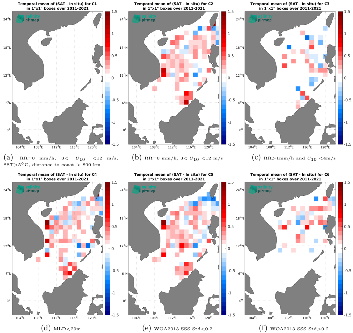
Figure 12: Temporal mean gridded over spatial boxes of size 1^\circ \times 1^\circ of \Delta\text{SSS} (SMOS SSS L3 v2 - 9-Days (BEC) - Argo) for 6 different subdatasets corresponding to: RR=0 mm/h, 3 < U_{10} < 12 m/s, SST > 5^\circ\text{C} , distance to coast > 800 km (a), RR=0 mm/h, 3 < U_{10} < 12 m/s (b), RR > 1 mm/h and U_{10} < 4 m/s (c), MLD < 20 m (d), WOA2013 SSS Std < 0.2 (e), WOA2013 SSS Std > 0.2 (f).
