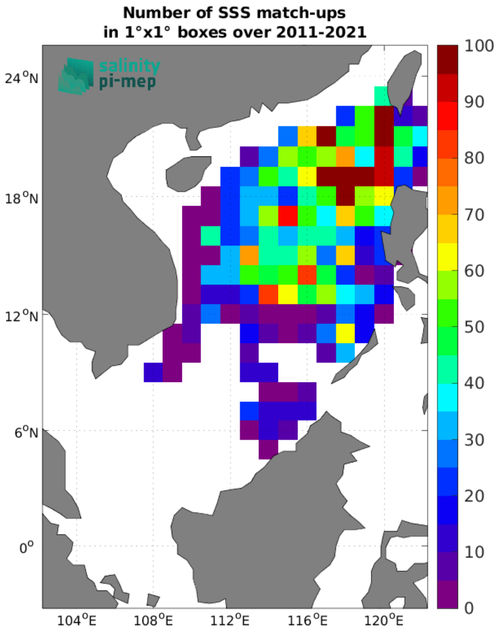
Figure 4: Number of SSS match-ups between Argo SSS and the SMOS SSS L3 v2 - 9-Days (BEC) SSS product for the South China Sea Pi-MEP region over 1^{\circ} \times 1^{\circ} boxes and for the full satellite product period.
