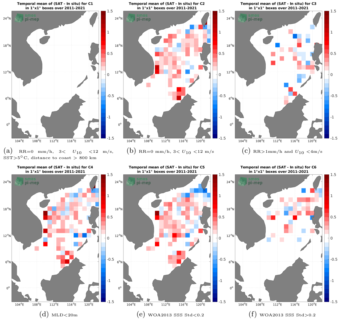
Figure 12: Temporal mean gridded over spatial boxes of size 1^\circ \times 1^\circ of \Delta SSS (SMOS SSS L3 v2 - 9-Days (BEC) - Argo) for 6 different subdatasets corresponding to:RR=0 mm/h, 3 < U_{10} < 12 m/s, SST>5°C, distance to coast > 800 km (a), RR=0 mm/h, 3 < U_{10} < 12 m/s (b), RR>1mm/h and U_{10} < 4 m/s (c),MLD<20m (d),WOA2013 SSS Std<0.2 (e),WOA2013 SSS Std>0.2 (f).
