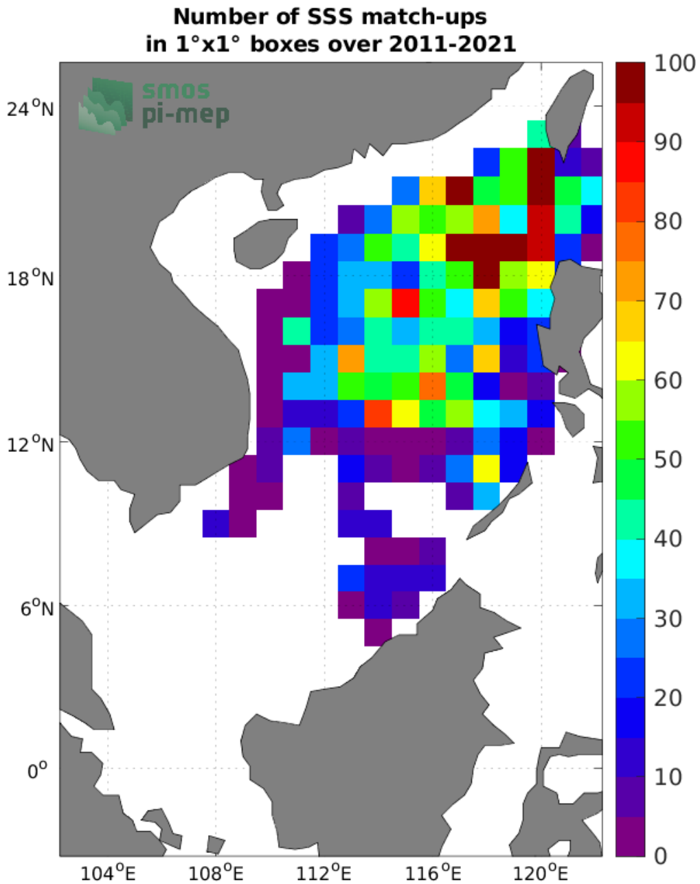
Figure 4: Number of SSS match-ups between Argo SSS and the SMOS SSS L3 v2 - 9-Days (BEC) SSS product for the South China Sea Pi-MEP region over 1^\circ \times 1^\circ boxes and for the full satellite product period.
