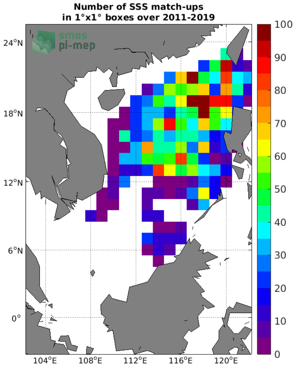
Figure 4: Number of SSS match-ups between Argo SSS and the SMOS SSS L3 v2 - 9-Days (BEC) SSS product for the South China Sea Pi-MEP region over 1°x1° boxes and for the full satellite product period.
