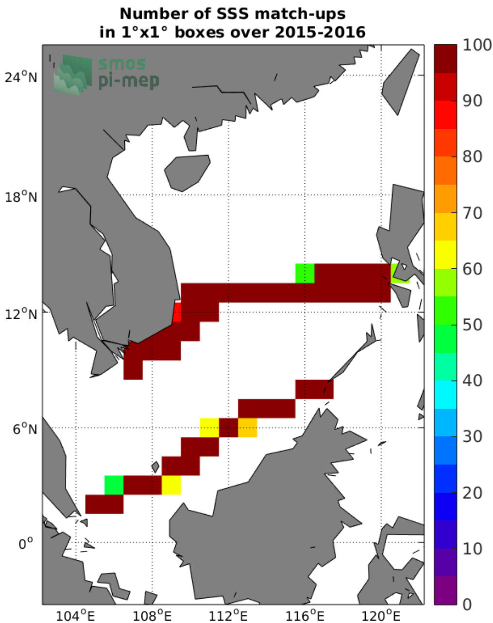
Figure 4: Number of SSS match-ups between TSG-SAMOS SSS and the SMOS-L3-BEC-OA-V1-9DAYS-0.25DEG SSS product for the South China Sea Pi-MEP region over 1°x1° boxes and for the full satellite product period.
