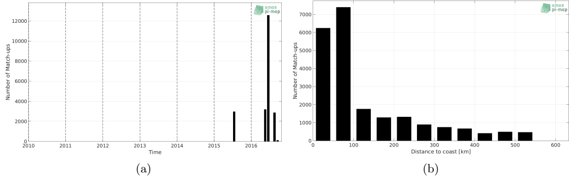
Figure 1: Number of match-ups between TSG-SAMOS and SMOS-L3-BEC-OA-V1-9DAYS-0.25DEG SSS as a function of time (a) and as function of the distance to coast (b) over the South China Sea Pi-MEP region and for the full satellite product period.
