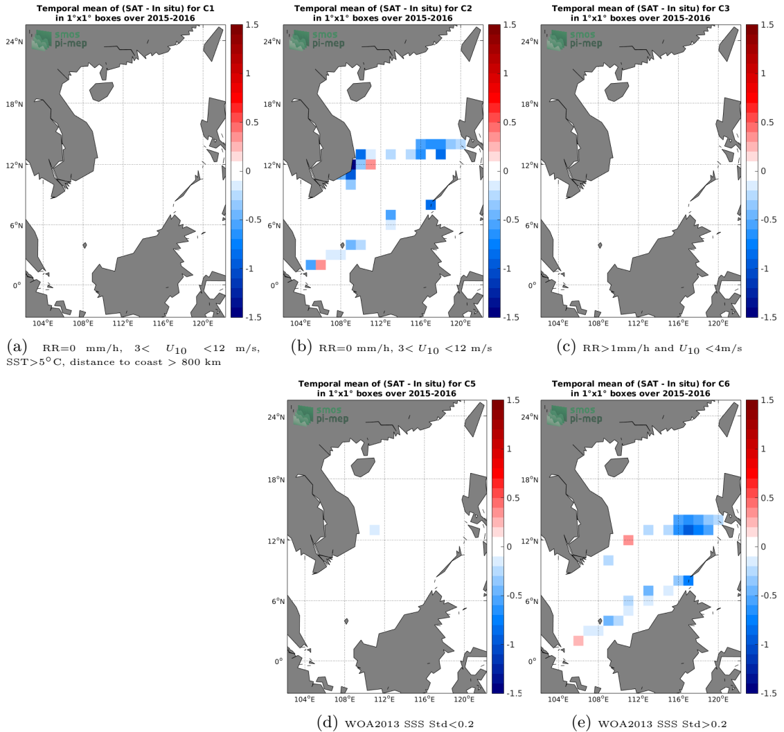
Figure 12: Temporal mean gridded over spatial boxes of size 1^\circ \times 1^\circ of \Delta SSS (SMOS-L3-BEC-OA-V1-9DAYS-0.25DEG - TSG-SAMOS) for 5 different subdatasets corresponding to:RR=0 mm/h, 3 < U_{10} < 12 m/s, SST>5°C, distance to coast > 800 km (a), RR=0 mm/h, 3 < U_{10} < 12 m/s (b), RR>1mm/h and U_{10} < 4 m/s (c), WOA2013 SSS Std<0.2 (d), WOA2013 SSS Std>0.2 (e).
