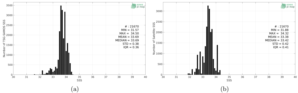
Figure 2: Histograms of SSS from TSG-SAMOS (a) and SMOS-L3-BEC-OA-V1-9DAYS-0.25DEG (b) considering all match-up pairs per bins of 0.1 over the South China Sea Pi-MEP region and for the full satellite product period.
