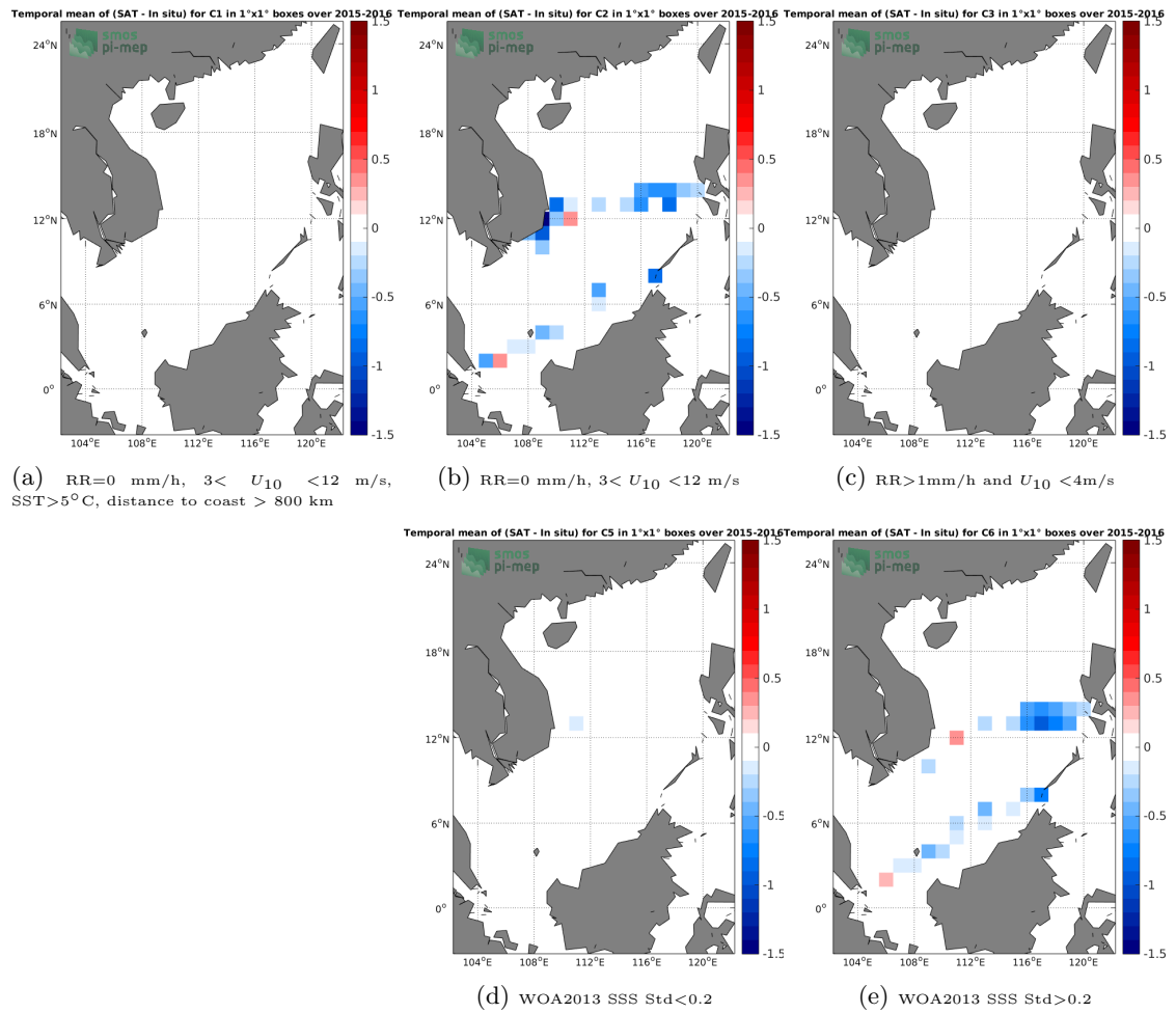
Figure 12: Temporal mean gridded over spatial boxes of size 1^\circ \times 1^\circ of \Delta SSS (SMOS-L3-BEC-OA-V1-9DAYS-0.25DEG - TSG-SAMOS) for 5 different subdatasets corresponding to: RR=0 mm/h, 3 < U_{10} < 12 m/s, SST > 5^\circ\text{C} , distance to coast > 800 km (a), RR=0 mm/h, 3 < U_{10} < 12 m/s (b), RR > 1 mm/h and U_{10} < 4 m/s (c), WOA2013 SSS Std < 0.2 (d), WOA2013 SSS Std > 0.2 (e).
