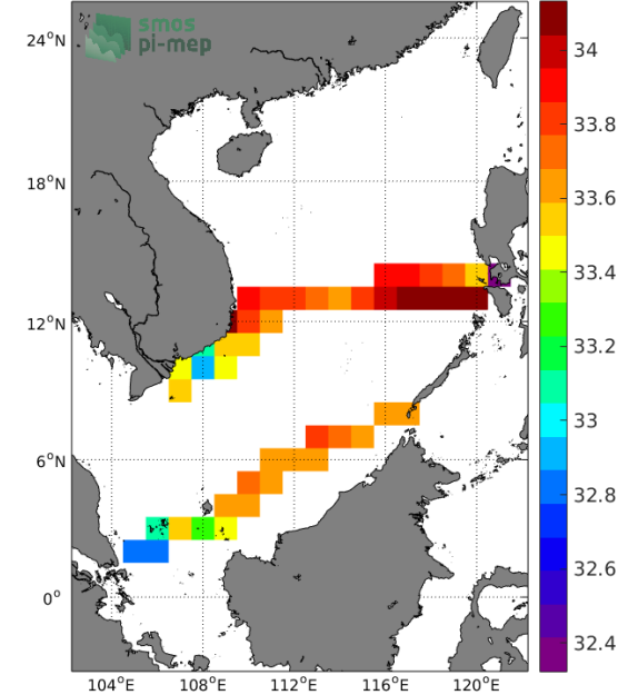
(c) MEAN(TSG-SAMOS SSS)
