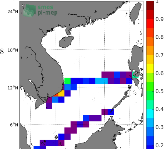
Temporal STD of (Sat-TSG-SAMOS) in 1°x1° boxes over 2015-2016
