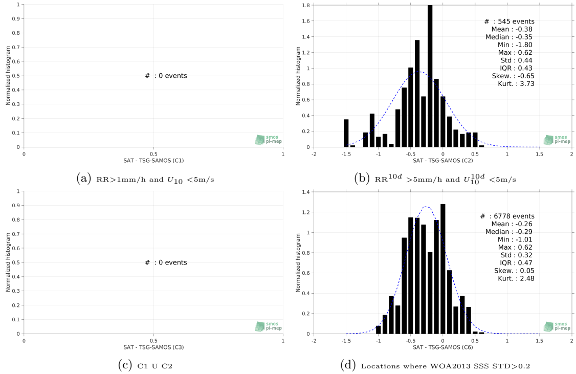
Figure 13: Normalized histogram of \Delta\text{SSS} (SMOS-L3-BEC-OA-V1-9DAYS-0.25DEG - TSG-SAMOS) for 6 different subdatasets corresponding to: RR > 1\text{mm/h} and U_{10} < 5\text{m/s} (a), RR^{10d} > 5\text{mm/h} and U_{10}^{10d} < 5\text{m/s} (b), C1 \cup C2 (c), Locations where WOA2013 SSS STD > 0.2 (d).
