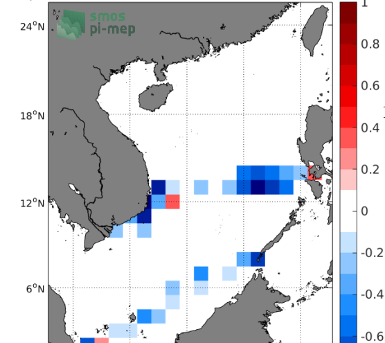
Temporal mean of (Sat-TSG-SAMOS) in 1°x1° boxes over 2015-2016
