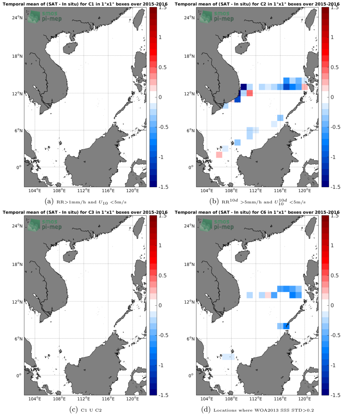
Figure 12: Temporal mean gridded over spatial boxes of size 1°x1° of \Delta\text{SSS} (SMOS-L3-BEC-OA-V1-9DAYS-0.25DEG - TSG-SAMOS) for 4 different subdatasets corresponding to: RR > 1\text{mm/h} and U_{10} < 5\text{m/s} (a), RR^{10d} > 5\text{mm/h} and U_{10}^{10d} < 5\text{m/s} (b), C1 U C2 (c), Locations where WOA2013 SSS STD > 0.2 (d).
