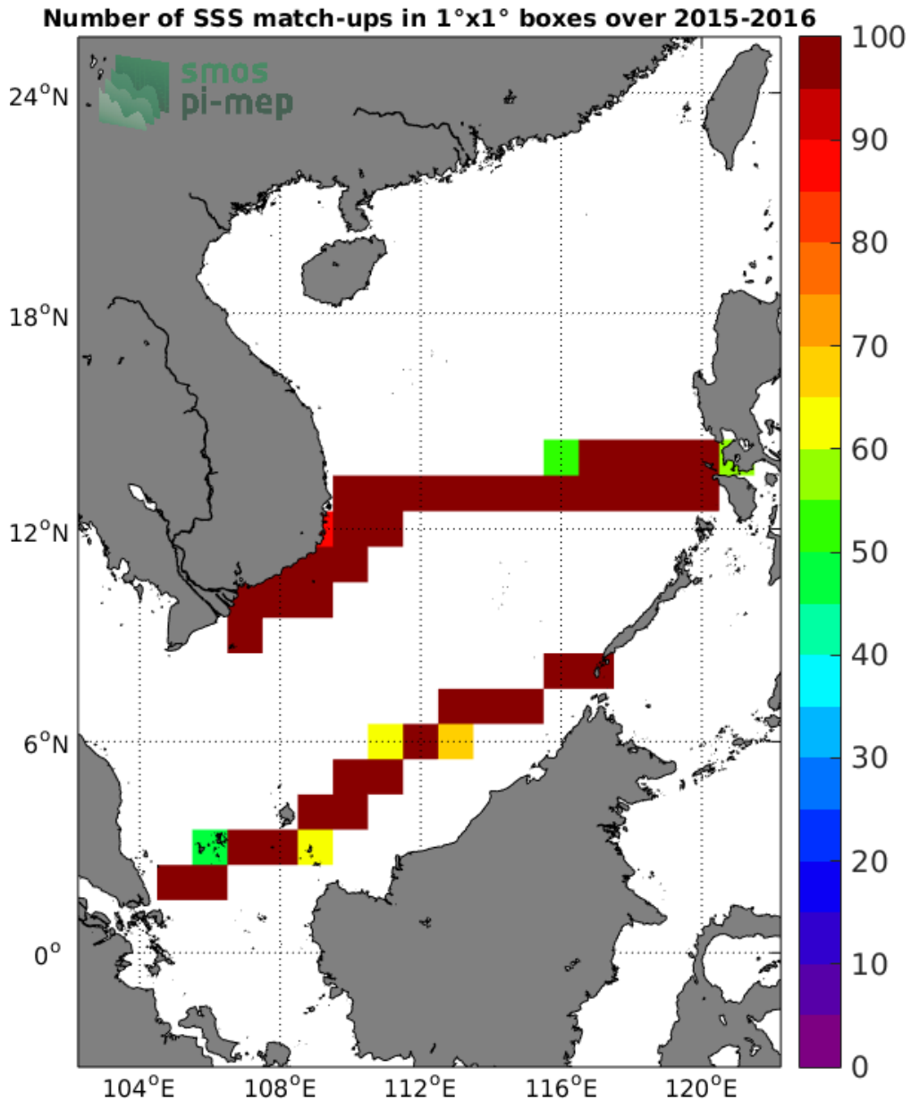
Figure 4: Number of SSS match-ups between TSG-SAMOS SSS and the SMOS-L3-BEC-OA-V1-9DAYS-0.25DEG SSS product for the South China Sea Pi-MEP region over 1°x1° boxes and for the full satellite product period.
