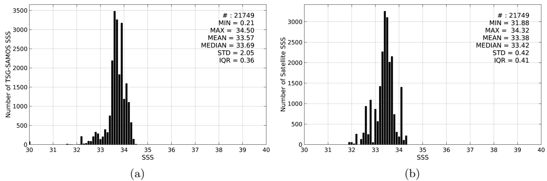
Figure 2: Histograms of SSS from TSG-SAMOS (a) and SMOS-L3-BEC-OA-V1-9DAYS-0.25DEG (b) considering all match-up pairs per bins of 0.1 over the South China Sea Pi-MEP region and for the full satellite product period.
