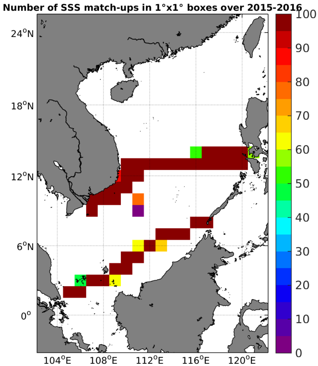
Figure 4: Number of SSS match-ups between TSG-SAMOS SSS and the SMOS-L3-BEC-OA-V1-9DAYS-0.25DEG SSS product for the South China Sea Pi-MEP region over 1°x1° boxes and for the full satellite product period.
