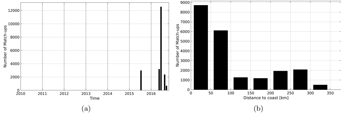
Figure 1: Number of match-ups between TSG-SAMOS and SMOS-L3-BEC-OA-V1-9DAYS-0.25DEG SSS as a function of time (a) and as function of the distance to coast (b) over the South China Sea Pi-MEP region and for the full satellite product period.
