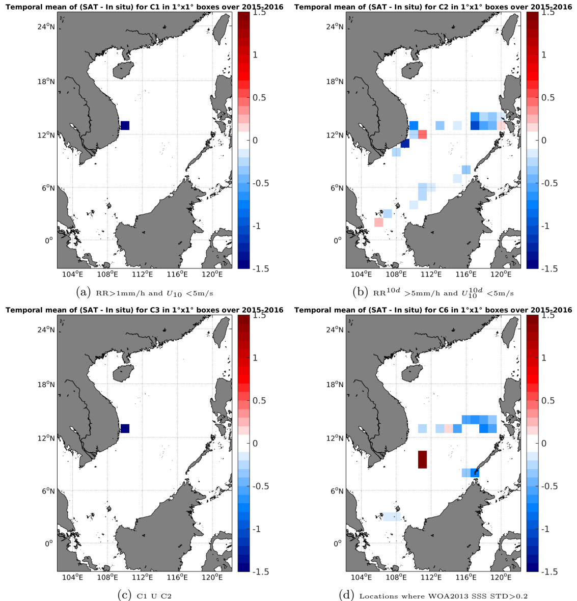
Figure 12: Temporal mean gridded over spatial boxes of size 1^\circ \times 1^\circ of \Delta SSS (SMOS-L3-BEC-OA-V1-9DAYS-0.25DEG - TSG-SAMOS) for 4 different subdatasets corresponding to:RR > 1 mm/h and U_{10} < 5 m/s (a), RR 10d > 5 mm/h and U_{10}^{10d} < 5 m/s (b), C1 U C2 (c),Locations where WOA2013 SSS STD > 0.2 (d).
