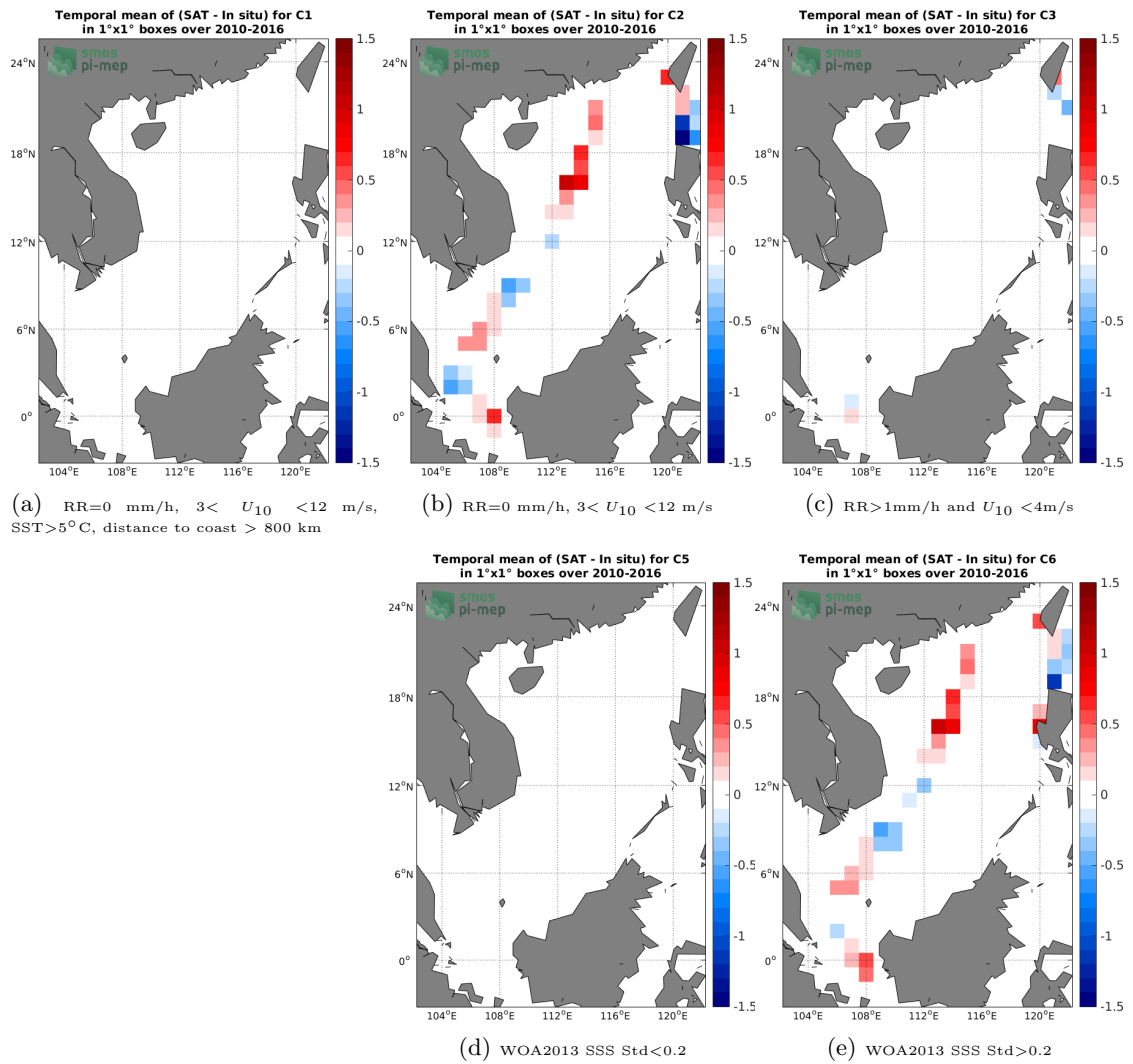
Figure 12: Temporal mean gridded over spatial boxes of size 1°x1° of \Delta SSS (SMOS-L3-BEC-OA-V1-9DAYS-0.25DEG - TSG-LEGOS-DM) for 5 different subdatasets corresponding to: RR=0 mm/h, 3 < U_{10} < 12 m/s, SST > 5^\circ C , distance to coast > 800 km (a), RR=0 mm/h, 3 < U_{10} < 12 m/s (b), RR > 1 mm/h and U_{10} < 4 m/s (c), WOA2013 SSS Std < 0.2 (d), WOA2013 SSS Std > 0.2 (e).
