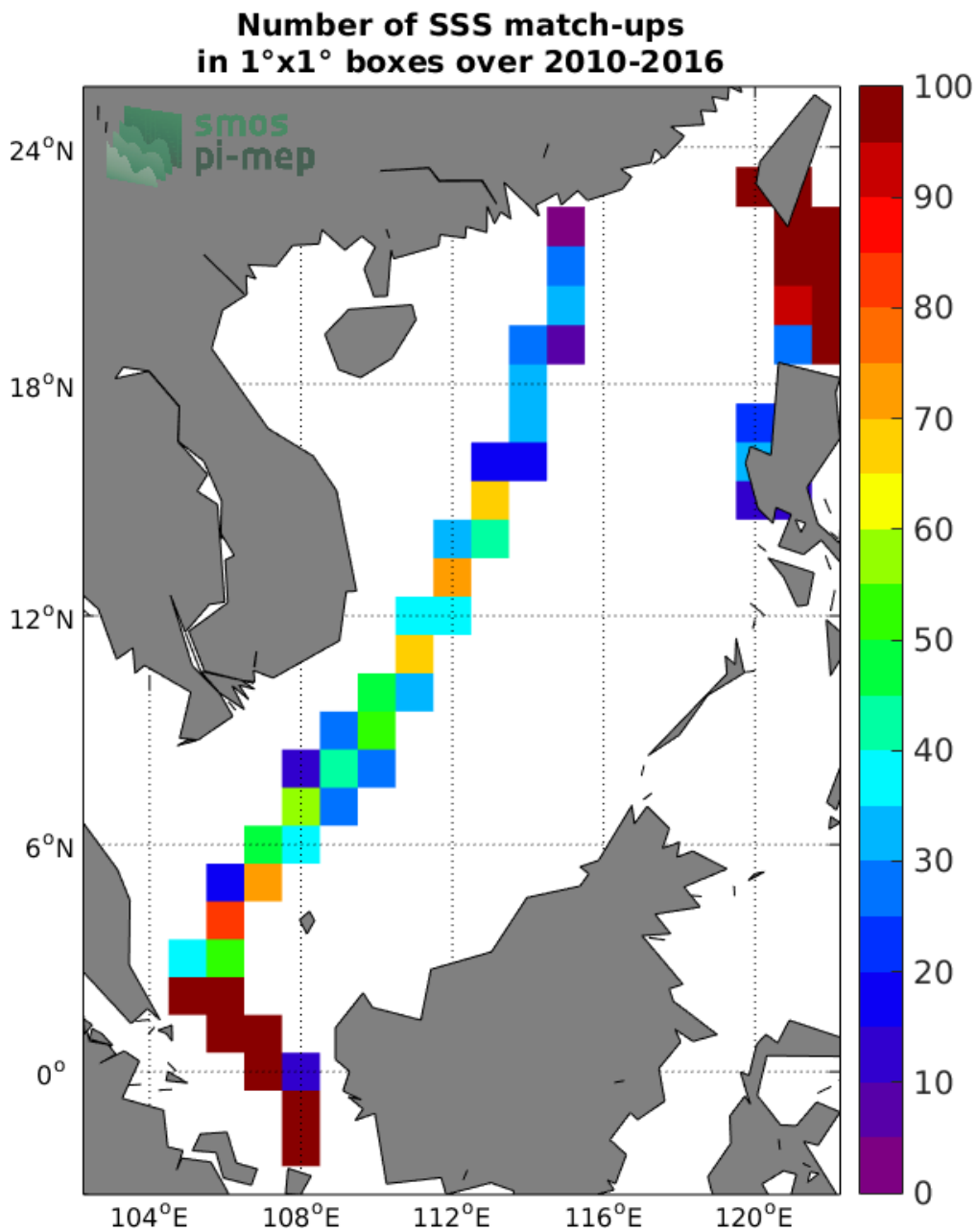
Figure 4: Number of SSS match-ups between TSG-LEGOS-DM SSS and the SMOS-L3-BEC-OA-V1-9DAYS-0.25DEG SSS product for the South China Sea Pi-MEP region over 1°x1° boxes and for the full satellite product period.
