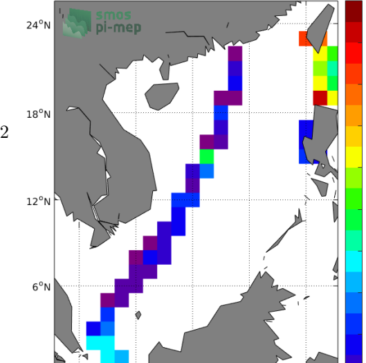
Temporal STD of (Sat-TSG-LEGOS-DM) in 1°x1° boxes over 2010-2016
