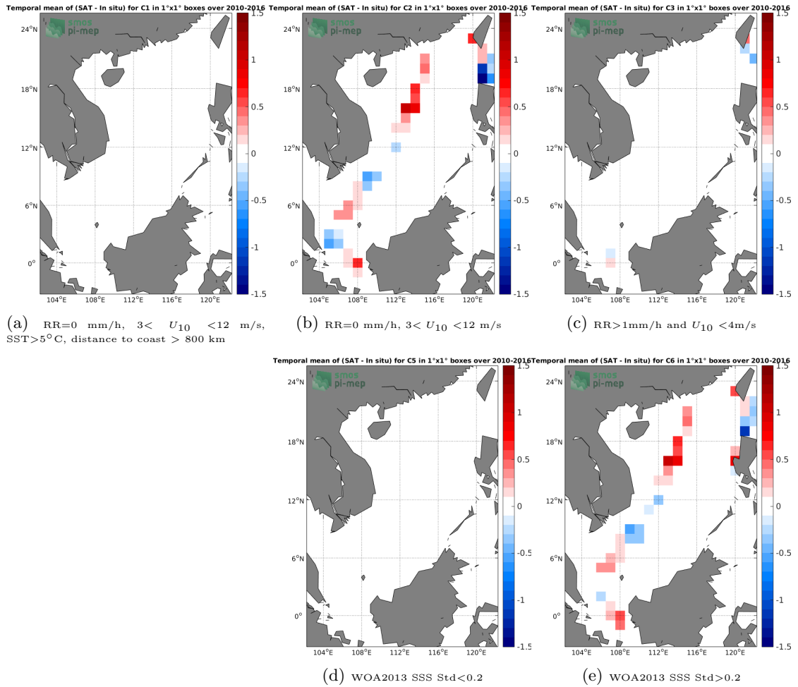
Figure 12: Temporal mean gridded over spatial boxes of size 1^\circ \times 1^\circ of \Delta SSS (SMOS-L3-BEC-OA-V1-9DAYS-0.25DEG - TSG-LEGOS-DM) for 5 different subdatasets corresponding to: RR=0 mm/h, 3 < U_{10} < 12 m/s, SST > 5^\circ C , distance to coast > 800 km (a), RR=0 mm/h, 3 < U_{10} < 12 m/s (b), RR > 1 mm/h and U_{10} < 4 m/s (c), WOA2013 SSS Std < 0.2 (d), WOA2013 SSS Std > 0.2 (e).
