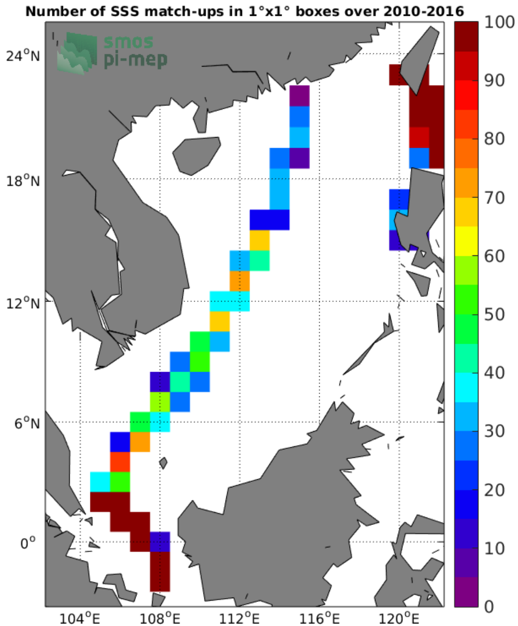
Figure 4: Number of SSS match-ups between TSG-LEGOS-DM SSS and the SMOS-L3-BEC-OA-V1-9DAYS-0.25DEG SSS product for the South China Sea Pi-MEP region over 1°x1° boxes and for the full satellite product period.
