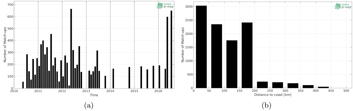
Figure 1: Number of match-ups between TSG-LEGOS-DM and SMOS-L3-BEC-OA-V1-9DAYS-0.25DEG SSS as a function of time (a) and as function of the distance to coast (b) over the South China Sea Pi-MEP region and for the full satellite product period.
