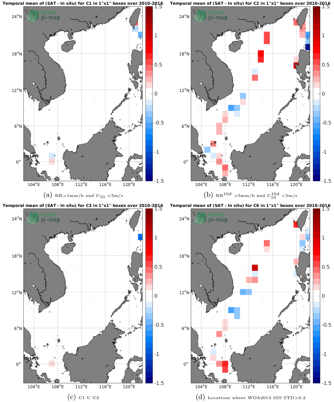
Figure 12: Temporal mean gridded over spatial boxes of size 1°x1° of \Delta\text{SSS} (SMOS-L3-BEC-OA-V1-9DAYS-0.25DEG - TSG-LEGOS-DM) for 4 different subdatasets corresponding to: RR > 1\text{mm/h} and U_{10} < 5\text{m/s} (a), RR^{10d} > 5\text{mm/h} and U_{10}^{10d} < 5\text{m/s} (b), C1 U C2 (c), Locations where WOA2013 SSS STD > 0.2 (d).
