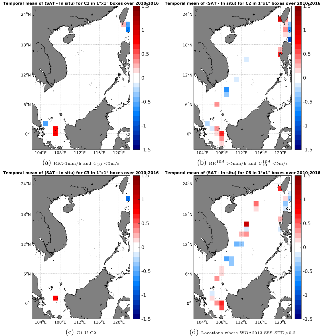
Figure 12: Temporal mean gridded over spatial boxes of size 1^\circ \times 1^\circ of \Delta SSS (SMOS-L3-BEC-OA-V1-9DAYS-0.25DEG - TSG-LEGOS-DM) for 4 different subdatasets corresponding to: RR > 1\text{mm/h} and U_{10} < 5\text{m/s} (a), RR^{10d} > 5\text{mm/h} and U_{10}^{10d} < 5\text{m/s} (b), C1 U C2 (c), Locations where WOA2013 SSS STD > 0.2 (d).
