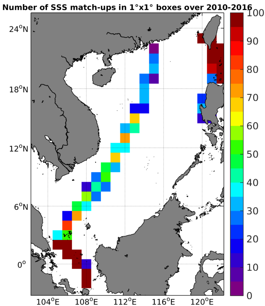
Figure 4: Number of SSS match-ups between TSG-LEGOS-DM SSS and the SMOS-L3-BEC-OA-V1-9DAYS-0.25DEG SSS product for the South China Sea Pi-MEP region over 1°x1° boxes and for the full satellite product period.
