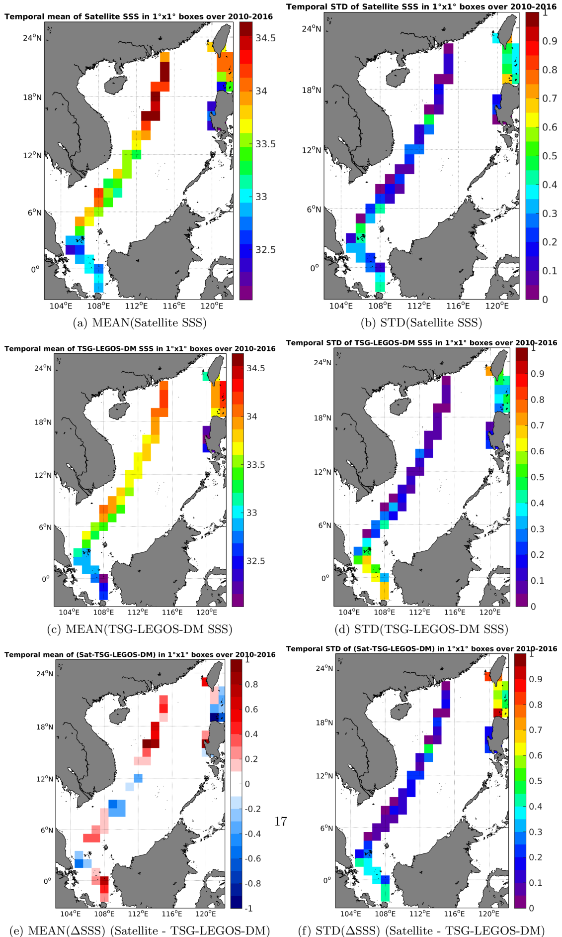
Figure 6: Temporal mean (left) and STD (right) of SSS from SMOS-L3-BEC-OA-V1-9DAYS-0.25DEG (top), TSG-LEGOS-DM (middle), and of \Delta SSS (Satellite - TSG-LEGOS-DM). Only match-up pairs are used to generate these maps.
