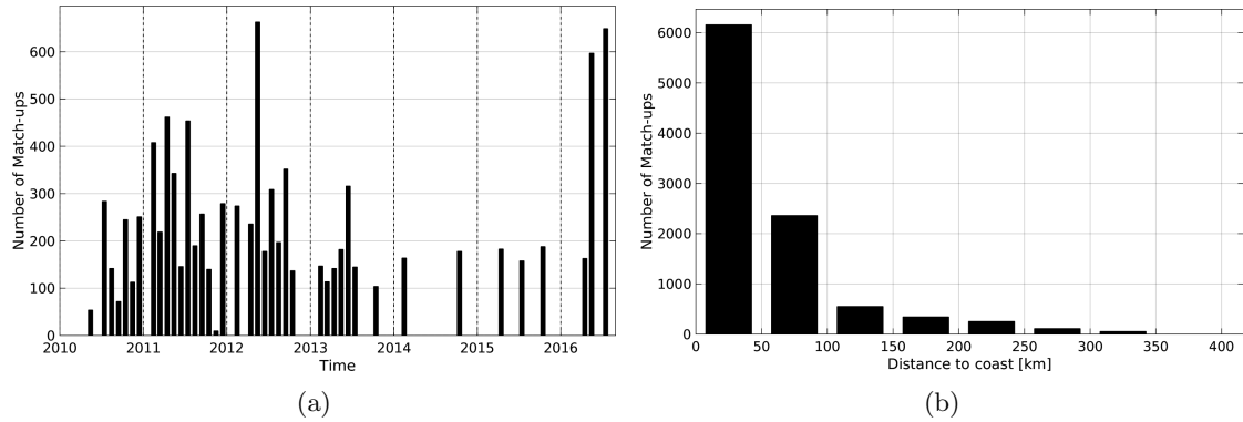
Figure 1: Number of match-ups between TSG-LEGOS-DM and SMOS-L3-BEC-OA-V1-9DAYS-0.25DEG SSS as a function of time (a) and as function of the distance to coast (b) over the South China Sea Pi-MEP region and for the full satellite product period.
