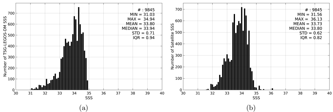
Figure 2: Histograms of SSS from TSG-LEGOS-DM (a) and SMOS-L3-BEC-OA-V1-9DAYS-0.25DEG (b) considering all match-up pairs per bins of 0.1 over the South China Sea Pi-MEP region and for the full satellite product period.
